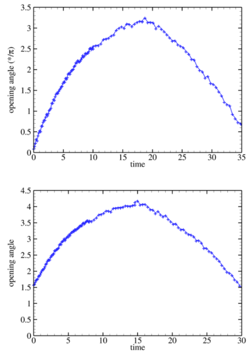
Figure 6. Time history of the opening angle using the pure stress-driven growth law without opening angle (a), and with the opening angle (b)
