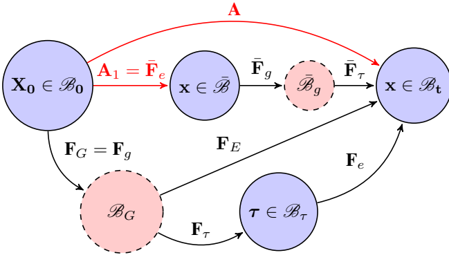
Figure 1. Growth from a stressed configuration \bar{\mathcal{B}} following a general deformation gradient \bar{\mathbf{A}}_1 = \bar{\mathbf{F}}_e . Then the body undergoes a small incremental deformation \bar{\mathbf{F}}_g , which is made compatible by \bar{\mathbf{F}}_\tau from \bar{\mathcal{B}}_g to \mathcal{B}_t . The result can be equally achieved following the lower path as \mathbf{F}_g from \mathcal{B}_0 to \mathcal{B}_g followed by \mathbf{F}_\tau from \mathcal{B}_g to \mathcal{B}_t , and then \mathbf{F}_e from \mathcal{B}_\tau to \mathcal{B}_t .
