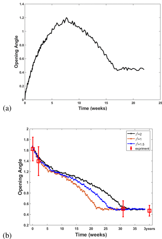
Figure 8. The time history of the opening angle using the mixed trigger growth law, with no initial opening angle (a), and with initial opening angle (b). The measured opening angles of young pigs' hearts from 1 day to 30 weeks and 3 years are shown as symbols and error bars in (b). It is noted that homeostasis is reached in all cases after 30 weeks. Furthermore, it appears that a value of \beta_I = 1.5 provides the best description of the experiments. Although values of 1 and 2 also yield qualitatively good results.
