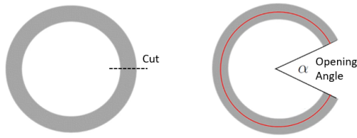
Figure 3. Definition of opening angle. Left: Drawing of a slice in the no-load state. The chamber centre of this configuration is estimated by constructing a diameter through the epicardial edge of the cut and the most distant epicardial point. Right: Same slice in the opening angle state. The opening angle is defined as the angle between the two radial lines connecting the centre of the ventricular chamber and the centre lines of the walls at the cut edges.
