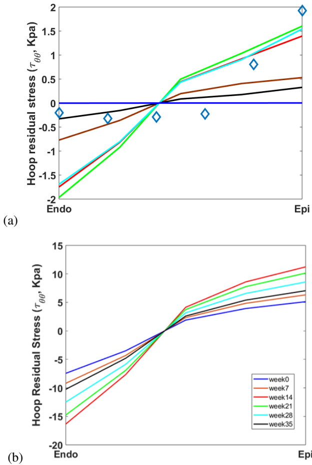
Figure 5. Transmural distributions of the hoop residual stress \tau_{\theta\theta} using the pure stress-driven growth law without opening angle (a), and with the opening angle (b). Blue-squared line represents the residual stress estimated by Wang et al. (2014) based on opening-angle experiment on heart by Costa et al. (1997)
