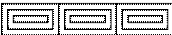
Pattern 7: Three reflections (two vertical, one horizontal)
