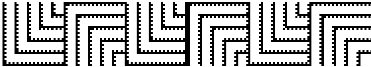
Pattern 3: Two parallel vertical reflections
