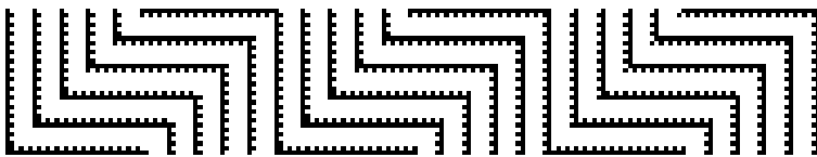
Pattern 5: A reflection and a half turn
