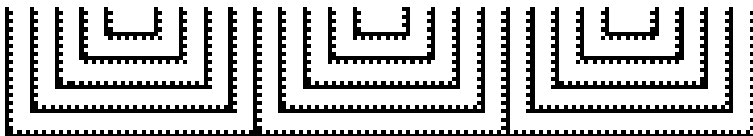
Pattern 4: Two half turns
