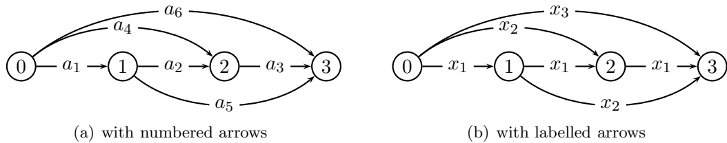
Figure 4.1: A labelled quiver of sections of \mathbb{P}(1, 2, 3) .
