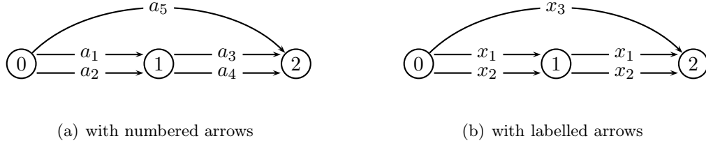
Figure 3.1: Quiver of sections of \mathbb{P}(1, 1, 2)
