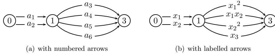
Figure 4.2: Abramovich-Hassett construction for \mathbb{P}(1, 1, 2) and n = 0, m = 2 .
