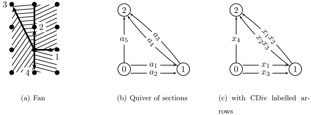
Figure 2.1: Hirzebruch surface \mathbb{F}_2
