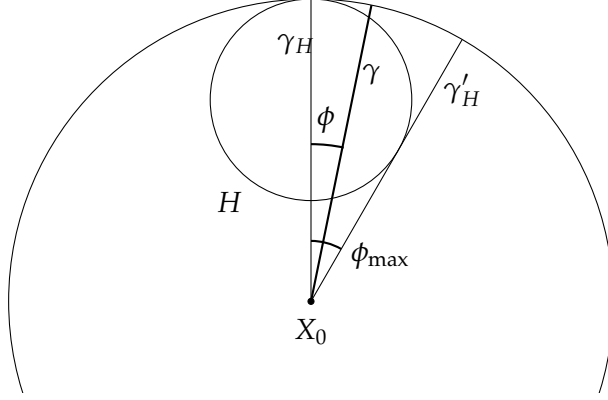
FIGURE 3.5. Excursion in the horoball H .
