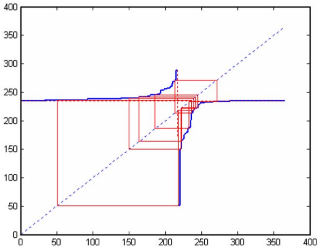
Fig. 10. G -function generated by adding 1^\circ\text{C} to observed phloem temperatures for Railroad Ridge, 1995. Horizontal axis is input oviposition date for the n th generation and the vertical axis is median ovipositional date for the (n+1) st generation (reduced modulo 365). Intersections with the dotted 1-1 fixed-point line (dashed) denote fixed points, which do not exist for this temperature series, indicating asynchrony. Cobwebbed iterates of the map, correspond to a complicated \frac{13}{20} orbit.
