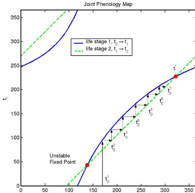
Fig. 2. Cobwebbing between first and second life stage curves to illustrate the dynamics of the joint two-stage phenology map. Julian days of emergence and oviposition appear on the horizontal axis, while Julian days of egg hatching appear on the vertical. A sequence of oviposition dates is generated by successive reflections between the first life stage output curve (solid) and the reflected second life stage output curve (dashed). A complete iteration from one generation to the next is accomplished by moving vertically from a given oviposition date to the solid curve (giving by its vertical displacement the output date from the first life stage) and then moving from that point horizontally to the dashed curve (giving by its horizontal displacement the output date from the second life stage). In this case, any sequence of oviposition dates will converge to the stable univoltine solution indicated by t^* . The other, unstable univoltine fixed point separates initial conditions between those which will converge to t^* from above and below.
