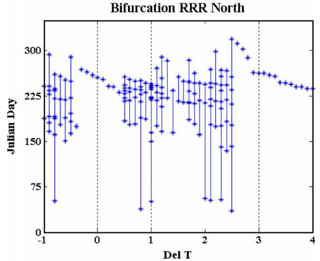
Fig. 7. Bifurcation plot for the annual temperatures cycle at Railroad Ridge, 1995. On the vertical axis appears Julian day of emergence, while horizontal axis indicates degrees Centigrade added to the 1995 temperature series. The observed temperature (blue in Fig. Ex1.1) is at x = \Delta T = 1 ; increasing the mean annual temperature by 1 °C added to each hourly observed temperature (green in Fig. Ex1.1) is indicated by the second dotted line; increasing the mean temperature by 3 °C added to each hourly observed temperature (red in Fig. Ex1.1) is indicated by the third dotted line.
