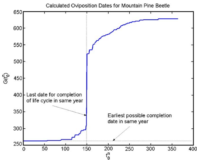
Fig. 3. Example G -function for Mountain Pine Beetle, calculated using recorded phloem temperatures in the Sawtooth National Recreation Area of central Idaho from 2002. Julian date of oviposition is plotted on the horizontal axis, and the number of days later that oviposition occurs appears on the vertical axis. The vertical asymptote around day 150 corresponds to the last date during 2002 for which an entire life cycle could be completed in the same year; the horizontal asymptote corresponds to the earliest possible emergence date in that year.
