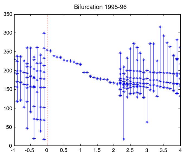
Fig. 16. Bifurcation plot of G -function iterates relative to the 1995 Stanley Basin temperature series. Amount of mean temperature added to every element of temperature series appears on horizontal axis in degrees Centigrade (so that 0 is the unperturbed 1995 temperature series); the last several iterates of the G -function are plotted on the vertical axis in Julian days. Unperturbed temperatures are at the beginning of a broad band of univoltine temperatures, indicating that continued warming should result in expanding growth of MPB populations.
