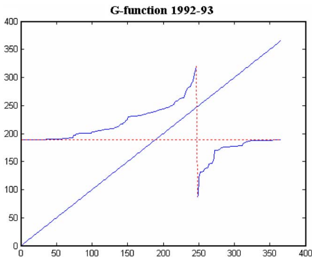
Fig. 14. G -function plot generated by 1992–93 temperatures in the Stanley Basin, during the Pinatubo perturbation. Julian days of oviposition in generation n and n + 1 are plotted on horizontal and vertical axes, respectively. Record low summer temperatures result in the nonexistence of univoltine fixed points and very late oviposition dates, making these temperatures maladaptive for mountain pine beetles. As a consequence, attacks on lodgepole pine were strongly suppressed during the summer of 1993.
