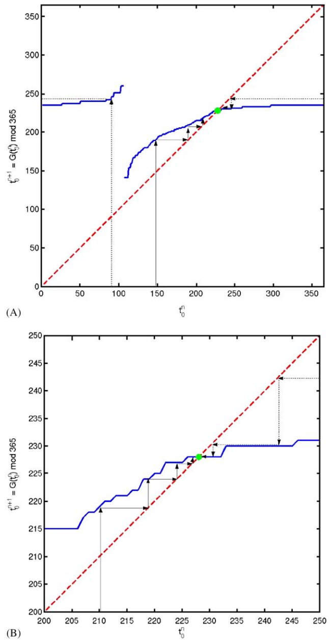
Fig. 4. Cobwebbing to illustrate the dynamic properties of the G -function. Julian days of oviposition in generation n and n+1 are plotted on horizontal and vertical axes, respectively. The solid curves above are oviposition dates in the next generation for given oviposition dates in the previous generation, plotted modulo 365. The dashed line is the t_0^{n+1} = t_0^n , and where it crosses the G -function, a univoltine fixed point exists, indicated by the solid circle. Dynamic iteration of the circle map results in reflections between the dashed and solid curves, as indicated by the arrows above. Two trajectories are illustrated, one in dotted and one in solid arrows, illustrating convergence to the fixed point from above and below. The second graph (B) is a blow-up of (A) for a range of dates close to the fixed point, illustrating the super-exponential convergence of trajectories to the fixed point in cases of quiescence (flat spots in the G -function).
