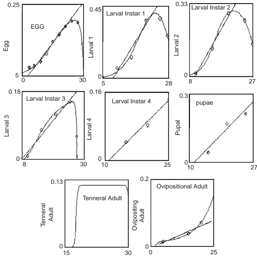
Fig. 5. Rate curves for the mountain pine beetle. In all curves, the vertical axis is measured in development/day and the horizontal axis is temperature in degrees Centigrade. Data points determined by rearing at controlled temperatures are depicted as open circles, and in some cases the location of a developmental threshold is estimated by using linear regression on a subset of the data points. Functional descriptions of the curves and best-fit parameter values are discussed in Jenkins et al. (2001).
