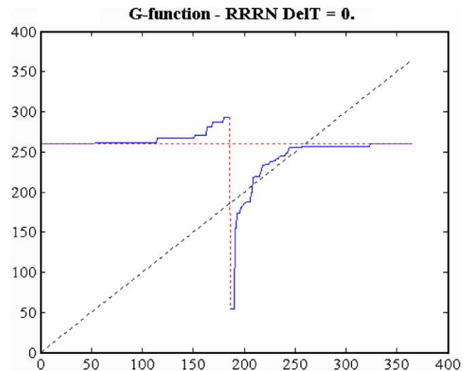
Fig. 8. G -function for the observed cycle of phloem temperatures for Railroad Ridge, 1995. Horizontal axis is input oviposition date for the n th generation and the vertical axis is median ovipositional date for the (n+1) st generation (reduced modulo 365). Intersections with the dotted 1–1 fixed-point line (dashed) indicate fixed points. In this case, the stable fixed point occurs around JD 250, in early September.
