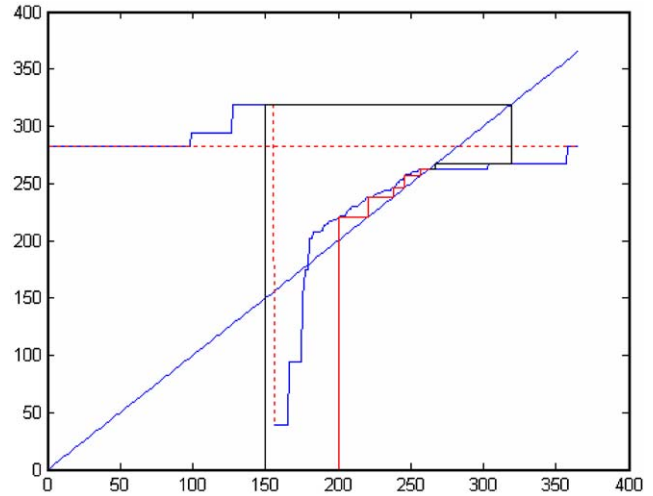
Fig. 11. G -function generated by adding 3^\circ\text{C} to phloem temperatures for Railroad Ridge, 1995. Horizontal axis is input oviposition date for the n th generation and the vertical axis is median ovipositional date for the (n+1) st generation (reduced modulo 365). Intersections with the dotted 1-1 fixed-point line (dashed) indicate fixed points. In this case, the stable fixed point occurs around JD 250, in early September. Cobwebbed iterates from an initial oviposition date of 200 are indicated in red.
