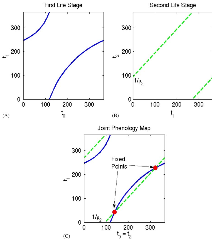
Fig. 1. Graphical representation of a simple two-stage phenology model, with output from the first stage graphed as solid lines (A), second stage output graphed as dashes (B), and the two graphs merged via identifying t_0 = t_2 from the second graph, resulting in an interchange of axes and the reflected plot of second stage output, appearing as a dashed line in (C). Where the dashed and solid curves intersect, a univoltine solution exists, indicated by the solid fixed points in the graph at left. Units on both horizontal and vertical axes are Julian days.
