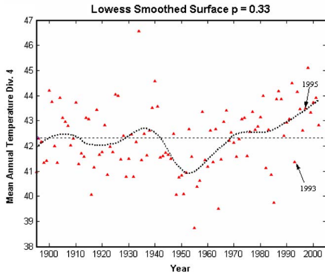
Fig. 17. Annual mean temperatures for NCDC Division 4, including the Stanley Basin, smoothed by a Robust Lowess Quadratic fit that includes a bracket of \frac{1}{3} of the data for each estimated smoothed point. Note the strong increasing trend from 1980 on and the relative position of the 1993 and 1995 years, well below and at the trend line, respectively.
