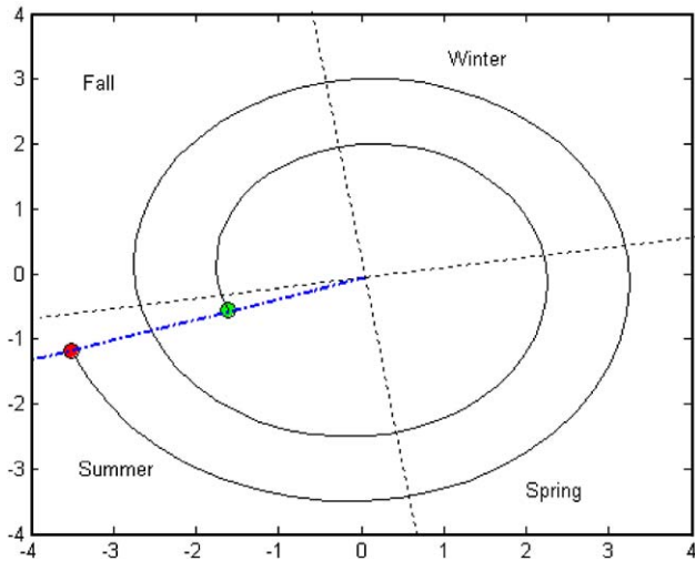
Fig. 9. Winding graph (nondimensional axes) of G -function iterates for the 1995 Railroad Ridge temperature series, where the scaled polar transformed starting ovipositional date (innermost circle) is plotted against the ending scaled polar-transformed median adult emergence date (red). The transformed date is scaled such that JD 1 translates to the (x,y) coordinates (0,1) , JD 365 translates to (0,2) , and so on. The winding number is (\text{number of fixed points plotted} - 1) / (\text{number of years}) . Fixed points attracting populations to oviposition at the same time of year (synchronous emergence) will result in points aligning on the radial vector (dash-dot line). Dotted lines correspond to solstices and equinoxes to indicate time of year.
