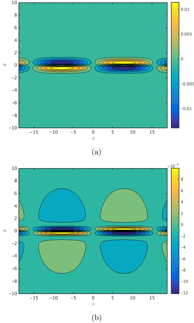
Figure 5. Optimal initial u_x for (a) t = 30 , (b) t = 40 .
