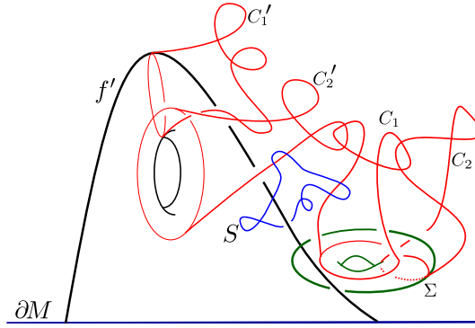
Figure 8. A single capped surface f' , whose caps intersect the caps of \Sigma . The dual sphere S for f' is produced by contraction of \Sigma .
