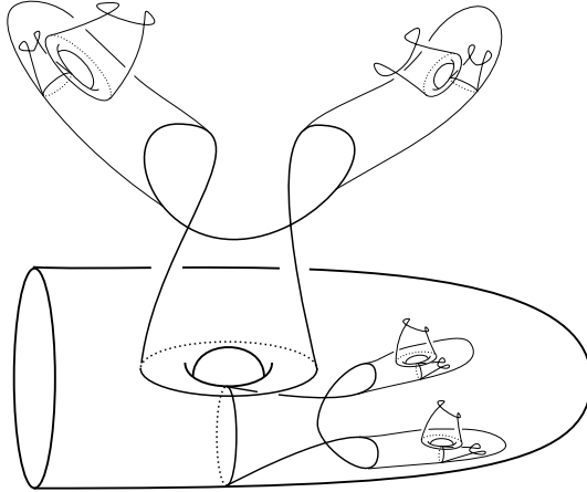
Figure 3. Schematic picture of the 2-dimensional spine of a 2-storey tower with one surface stage in each storey.
