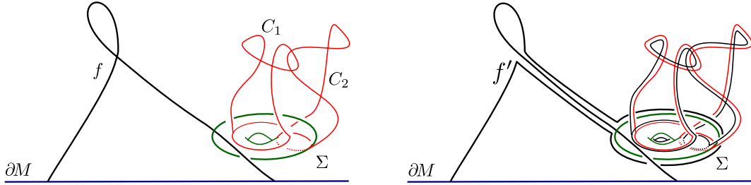
Figure 7. Producing capped surfaces. The self-intersection of the disc f (black) is tubed into the dual capped surface \Sigma (green). This disc is thus converted into a capped surface, when endowed with parallel copies of the caps for \Sigma .
