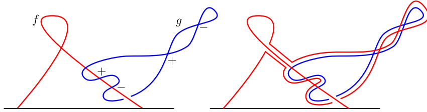
Figure 16. Modify f using g to get \mu(f) = 0 .
