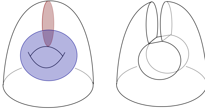
Figure 4. (Symmetric) contraction of a capped surface. Here we show the situation for embedded caps.
