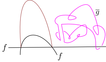
Figure 20. An embedded Whitney disc whose interior is in the complement of f and \bar{g} has been produced.
