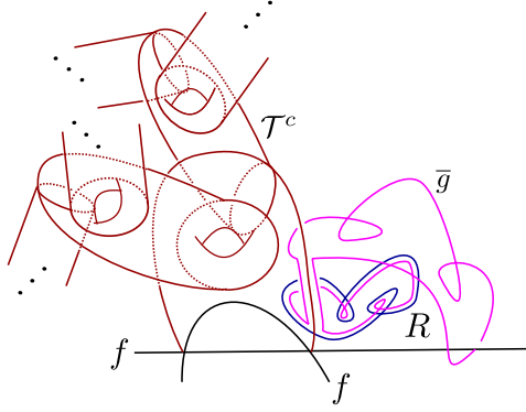
Figure 19. Tube to remove intersections of g with \mathcal{T}^c , ensuring that the interior of \mathcal{T}^c lies in the complement of f and \bar{g} .
