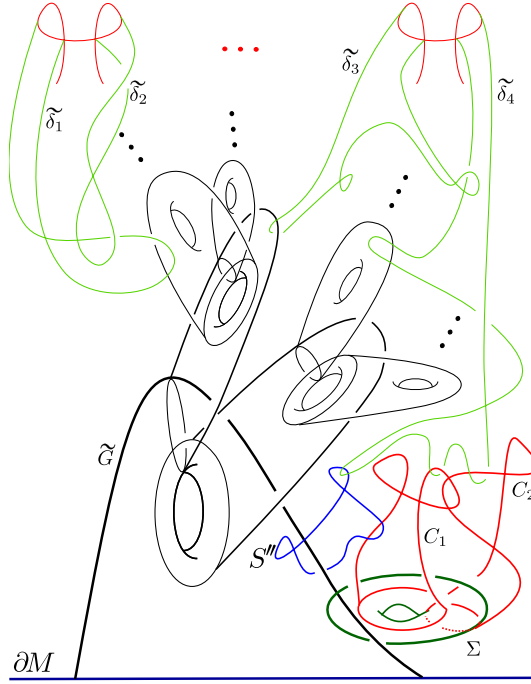
Figure 14. Obtaining discs (light green) from null homotopies of the double point loops. We have produced a dual sphere S'' (blue) for \tilde{G} (black).
