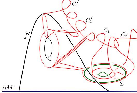
Figure 11. Push down the cap intersections of f' and tube into the dual capped surface.
