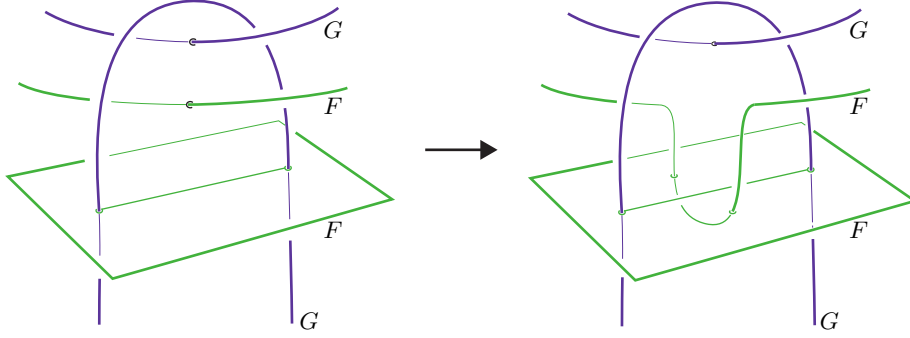
Figure 6. Pushing down a sheet of F into itself.
