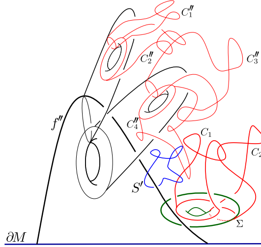
Figure 12. A dual sphere S' for f'' has been produced.
