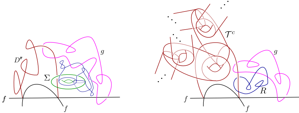
Figure 18. Before (left) and after (right) applying Proposition 6.5 to M \cup \nu f_i =: M' .
