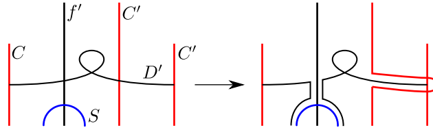
Figure 9. Separating the caps of \{\Sigma_i\} and \{f'_i\} .
