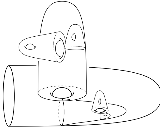
Figure 1. Schematic picture of the 2-dimensional spine of a height three grope.
