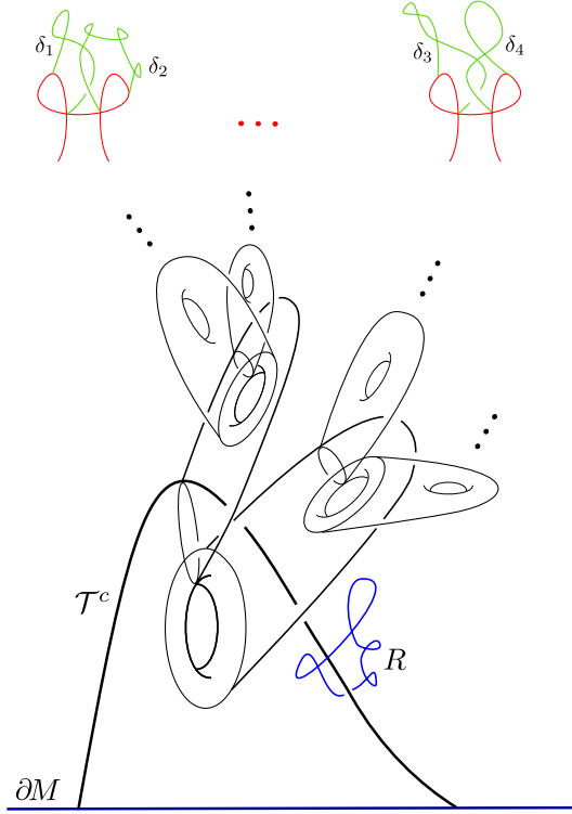
Figure 15. A 1-storey capped tower \mathcal{T}^c with a geometrically dual sphere R .
