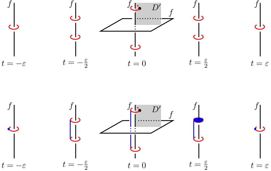
Figure 17. The top shows a (red) Clifford torus with a single intersection point with the (grey) Whitney disc D' pairing intersection points of f (black). In the bottom we see that each (blue) meridional disc intersects exactly one f_i once.
