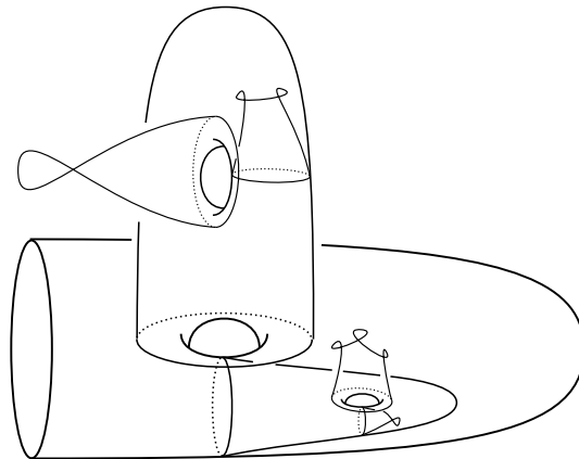
Figure 2. Schematic picture of the 2-dimensional spine of a height two capped grope.
