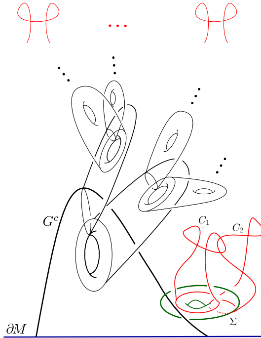
Figure 13. The result of grope height raising followed by the sequential contraction lemma. The caps of \Sigma may have changed by a regular homotopy of the interior.
