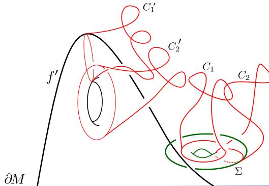
Figure 10. After separating the caps of \{\Sigma_i\} and \{f'_i\} .
