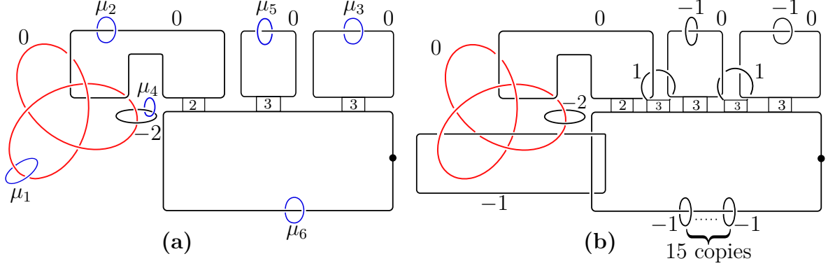
Figure 4.1: (a) Kirby diagram for the 4-manifold Z , (b) Kirby diagram showing an embedding of Z into K_3 \# 2\overline{\mathbb{CP}}^2 .
