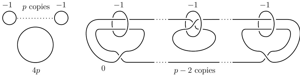
Figure 9.1: On the left: a surgery diagram for Y \# (\#^p S^3) . On the right: the surgery diagram after performing the handle slides described in the proof of Lemma 9.4.1.
