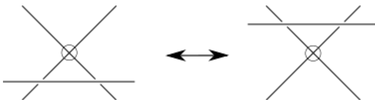
Figure 7.7: Overcrossing on welded braids.
