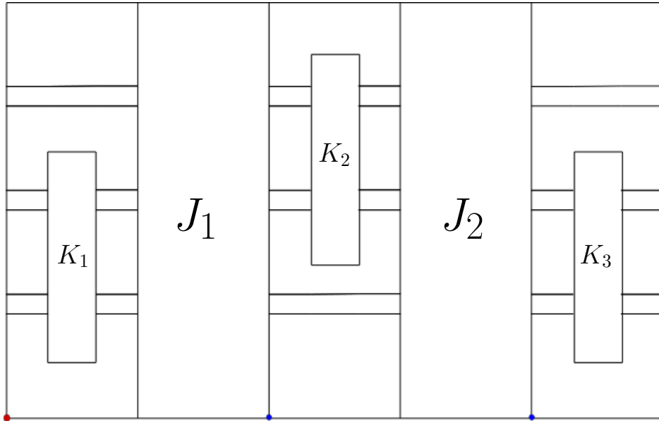
Figure 7.9: A schematic for the proof of Theorem 7.1.24 where the red point represents the basepoint we want to make our calculations from and the blue represent the basepoints we use to make our initial calculations of the intersections of K_i before we then rebase and use the isomorphism induced by the stack of singular pure braids to the left of the basepoint.
