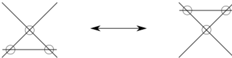
Figure 7.5: The third virtual Reidemeister move.
