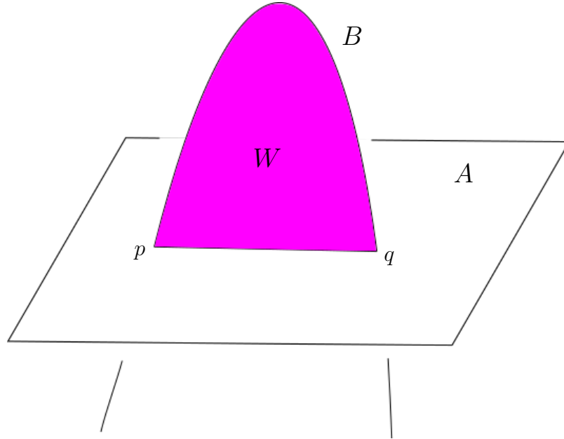
Figure 3.2: A local picture of a framed embedded Whitney disc W , pairing the intersections p and q , with sheet A lying in the present and sheet B having a arc lying in the present and the rest going into the past and future.
