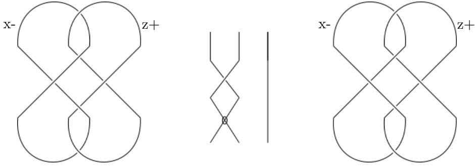
Figure 7.8: A description of a non-trivial three-component link map, where, at the top of the welded braid, the leftmost strand represents the x component, the centre strand represents the y component and the rightmost stand represents the z component. Also the orientations on each strand point down towards the bottom of the diagram.
