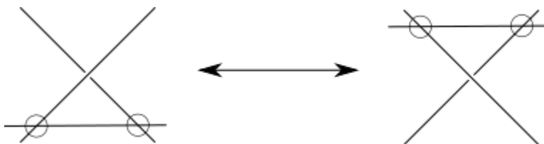
Figure 7.6: The fourth virtual Reidemeister move.
