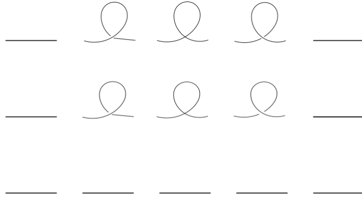
Figure 3.4: A description of a cusp homotopy
