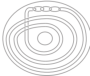
Fig. 1. A (4, 3) -link with the meridian of the solid torus omitted
