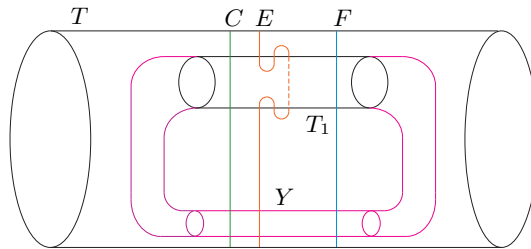
Fig. 2. Adding a cylinder Y to build a solid torus intersecting C, E and F (at least) twice each
