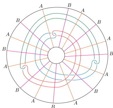
Fig. 6. A (3, 2) -link with an 8-interlacing. In this case D_L(8) = 10
