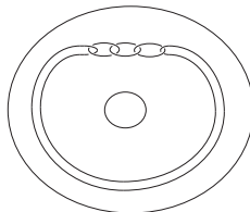
Fig. 4. A (4, 1) -link as a sublink of the 3-fold covering link \widetilde{J} of the (4, 3) -link from Figure 1
