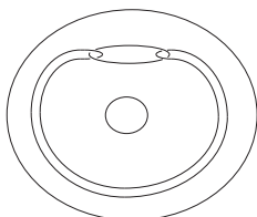
Fig. 5. The link J obtained by blowing down two of the components of the link of Figure 4. With the meridian of the solid torus, this is the Borromean rings with a clasp changed.
