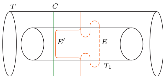
Fig. 3. Altering the interlacing disc E to E' , so that the intersection E' \cap T_1 is a meridional disc
