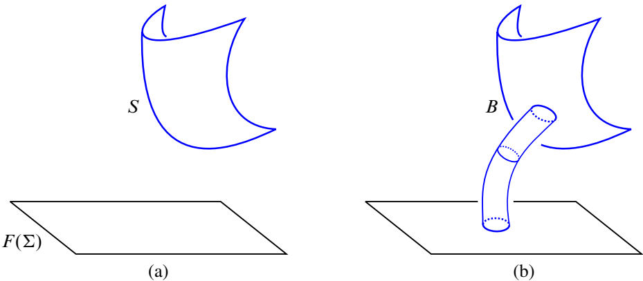
Figure 6: (a) An immersed surface S (blue) in the ambient manifold M , and the image (black) of a generic immersion F: (\Sigma, \partial \Sigma) \looparrowright (M, \partial M) . (b) A thin tube is added, with one boundary component on \Sigma and one on S . The surface B (blue) is obtained by cutting out a disc on S and gluing in the tube. Note that, compared to S , the surface B has a new boundary component lying on \Sigma .
