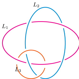
FIGURE 14. The link L8a16 .
