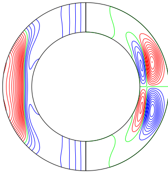
\bar{u}_\varphi & merid circulation (mer)
