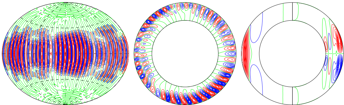
u_r at r = 0.9
