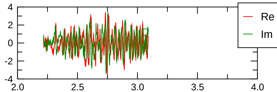
\text{tor}(m=0) magn.
