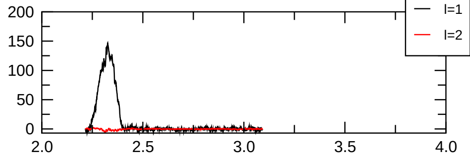
\text{pol}(m=2) magn.
