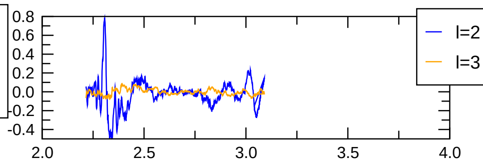
\text{pol}(m=0) magn.
