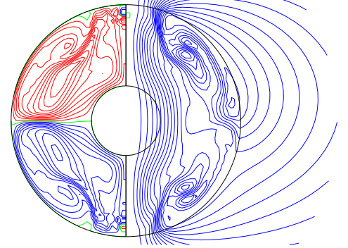
\bar{B}_\phi & pol f-lines (mer)
