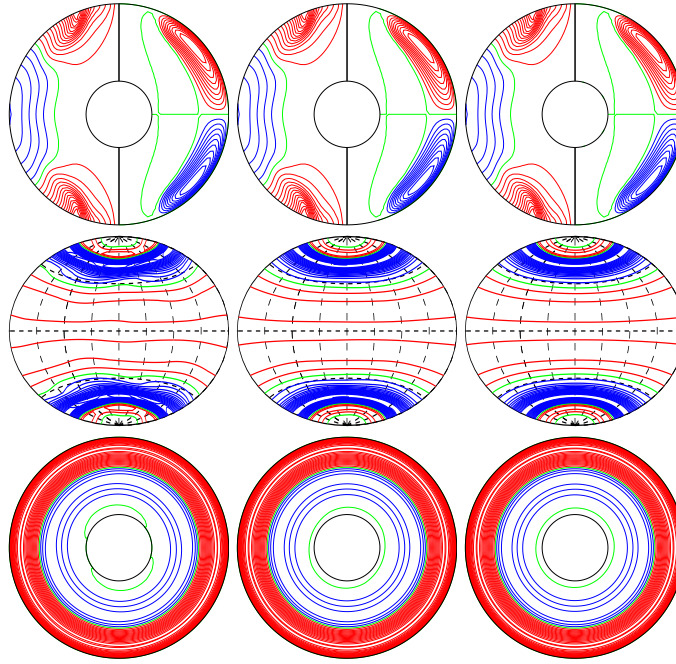
a.e03p1t03r-10m1n2N5z1.25e5 E_{\text{kin}}
