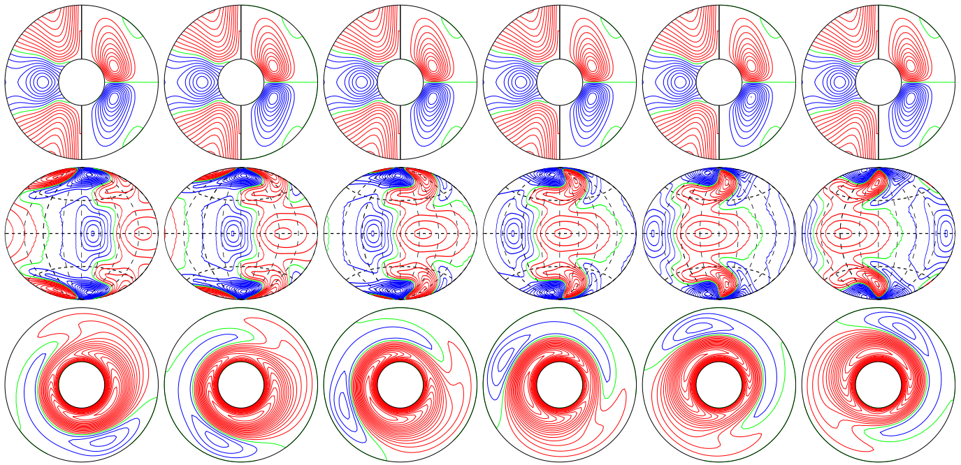
a.e03p1t03r-10m1n2N0001z1.25e5 E_{\text{kin}}
