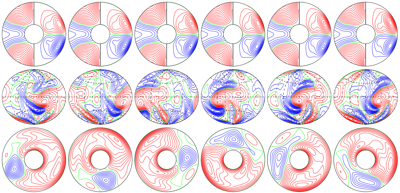
a.e03p1t03r-1000m1n2N1z1.25e5 E_{\text{kin}}
