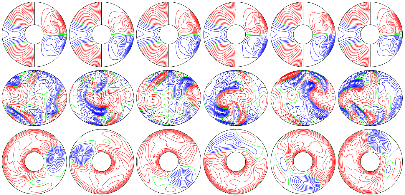
a.e03p1t03r-10m1n2N1z1.228e5 E_{\text{kin}}
