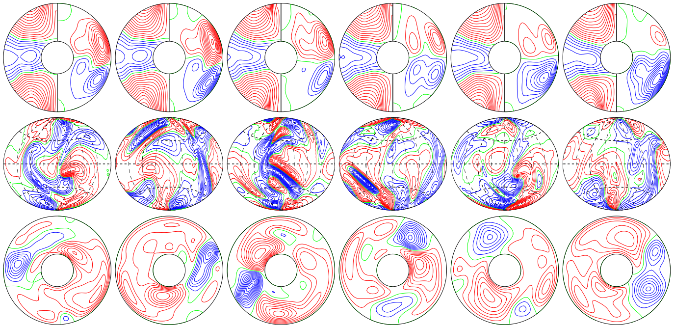
a.e03p1t05r-10m1n2N1z3.2e5 E_{\text{kin}}
