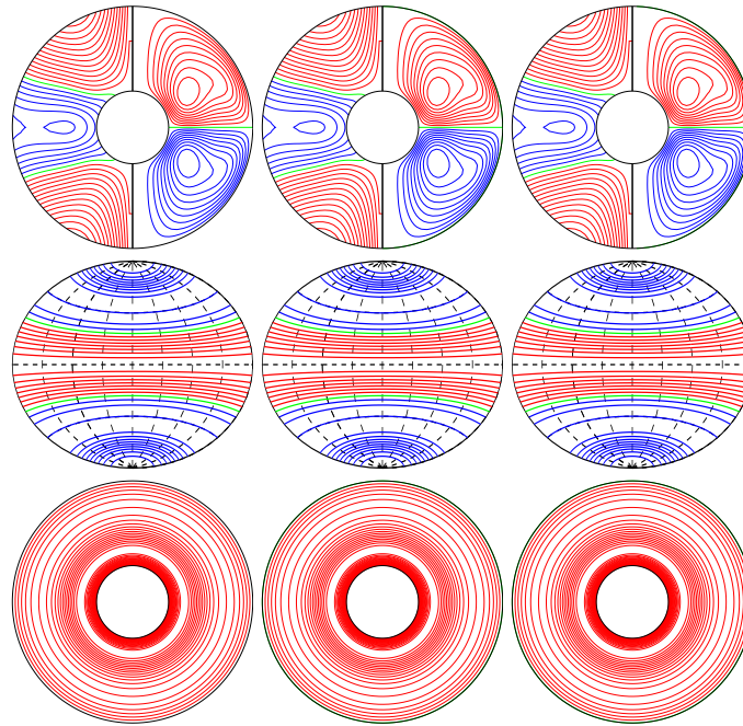
a.e03p1t03r-10m1n2N1z8e4 E_{\text{kin}}
