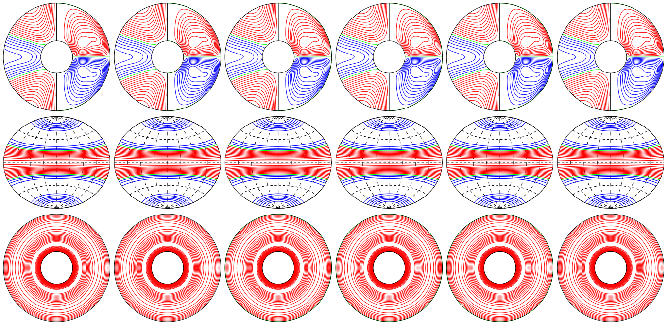
a.e03p1t03r-10m1n2N1z1.1e5 E_{\text{kin}}
