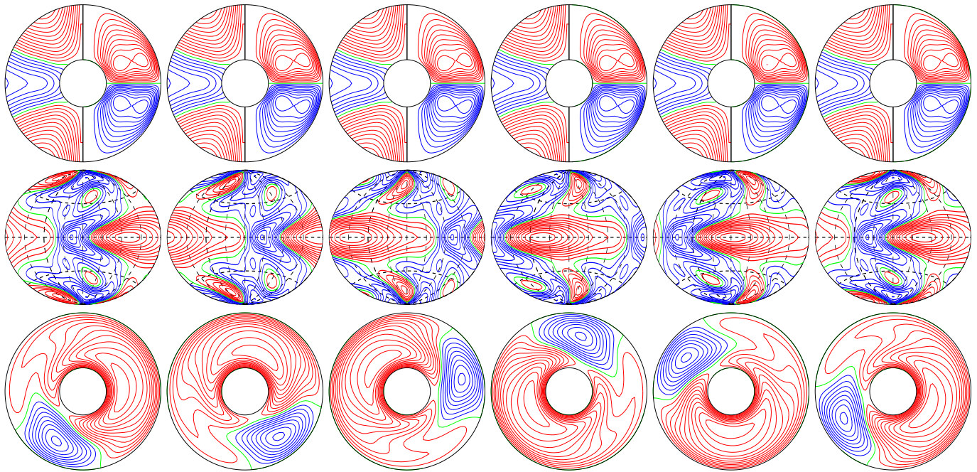
a.e03p1t03r-10m1n2N1z1.222e5 E_{\text{kin}}
