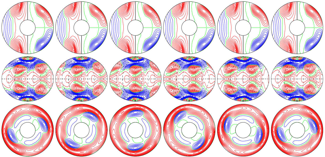
a.e03p1t03r-10m1n2N3z1.4e5 E_{\text{kin}}
