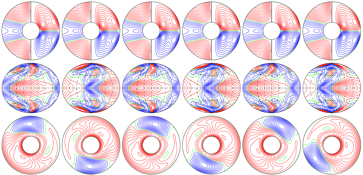
a.e03p1t05r-10m1n2N1z2.9e5 E_{\text{kin}}
