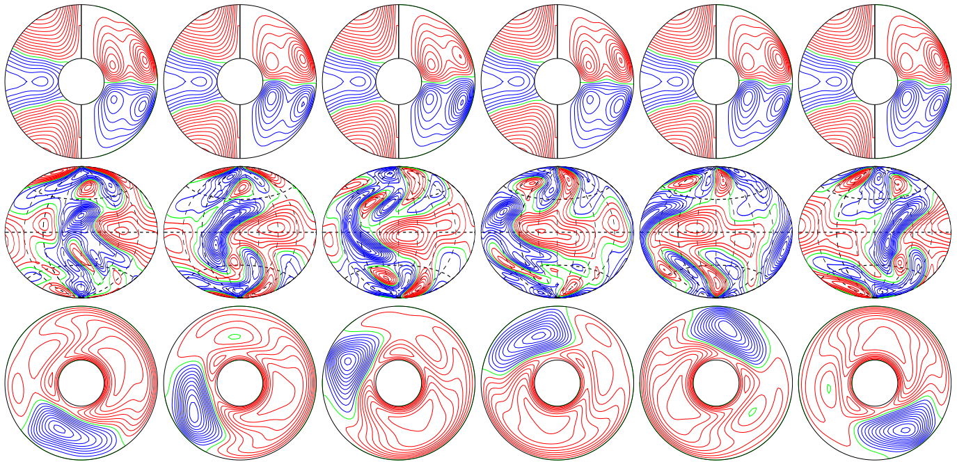
a.e03p1t05r-10m1n2N1z3.01e5 E_{\text{kin}}
