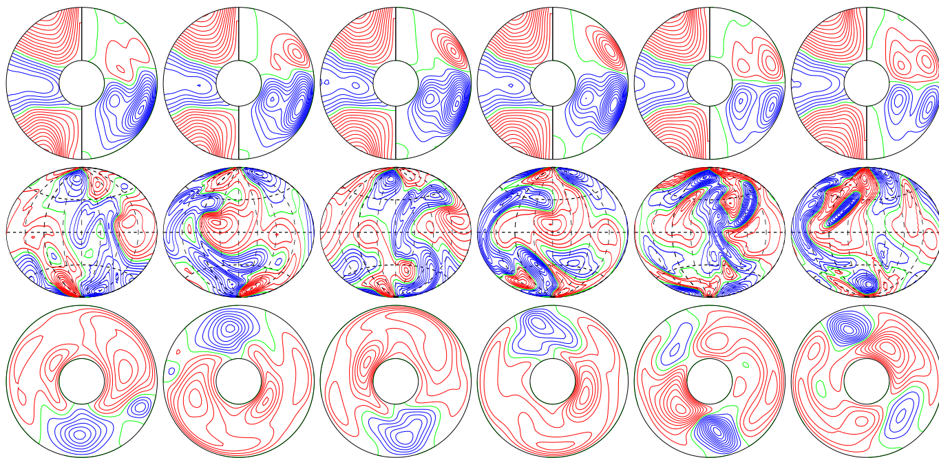
a.e03p1t05r-10m1n2N1z3.15e5 E_{\text{kin}}
