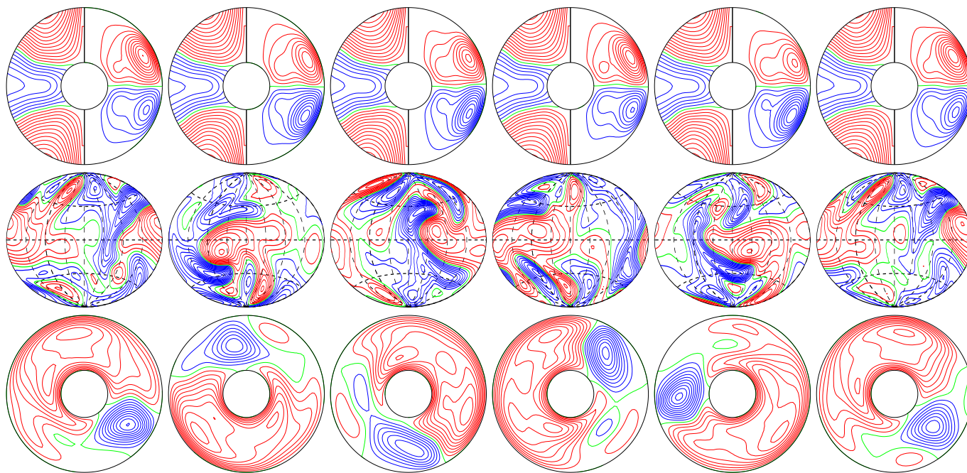
a.e03p1t03r-10m1n2N1z1.226e5 E_{\text{kin}}
