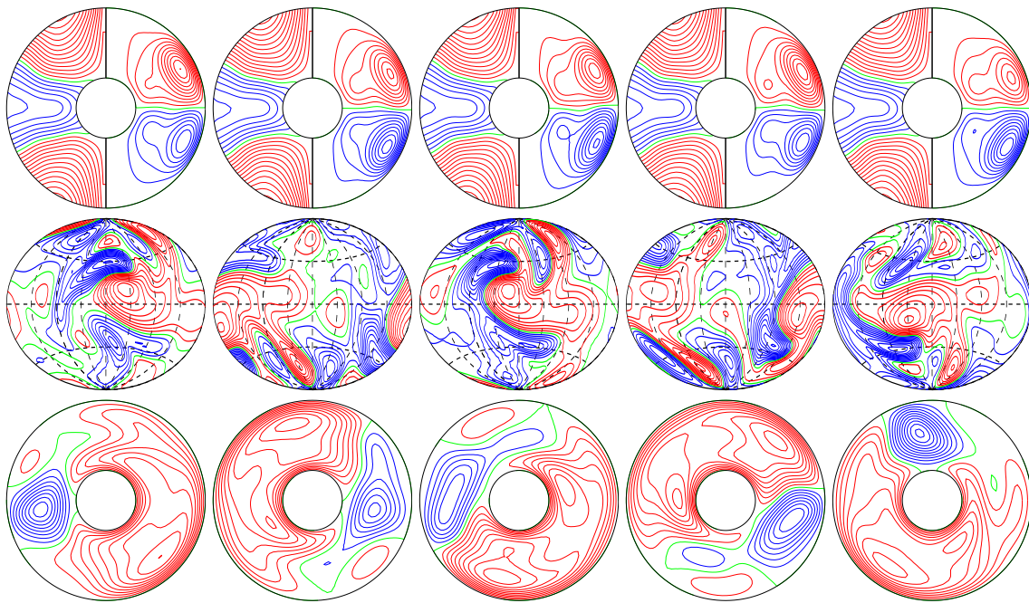
a.e03p1t03r-10m1n2N1z1.23e5 E_{\text{kin}}
