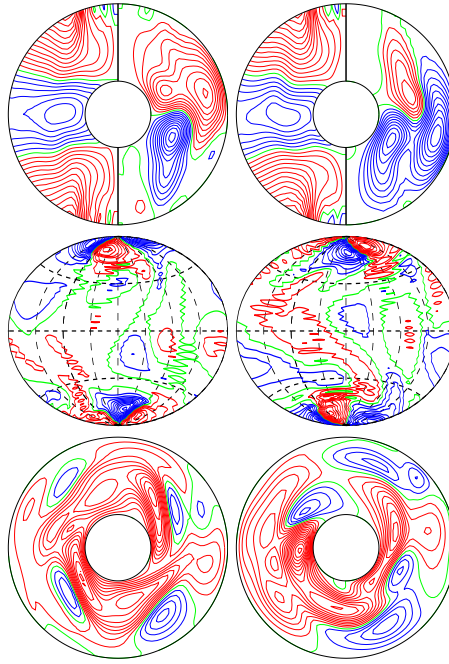
a.e03p1t1r-10m1n2N1z1.08e6 E_{\text{kin}}
