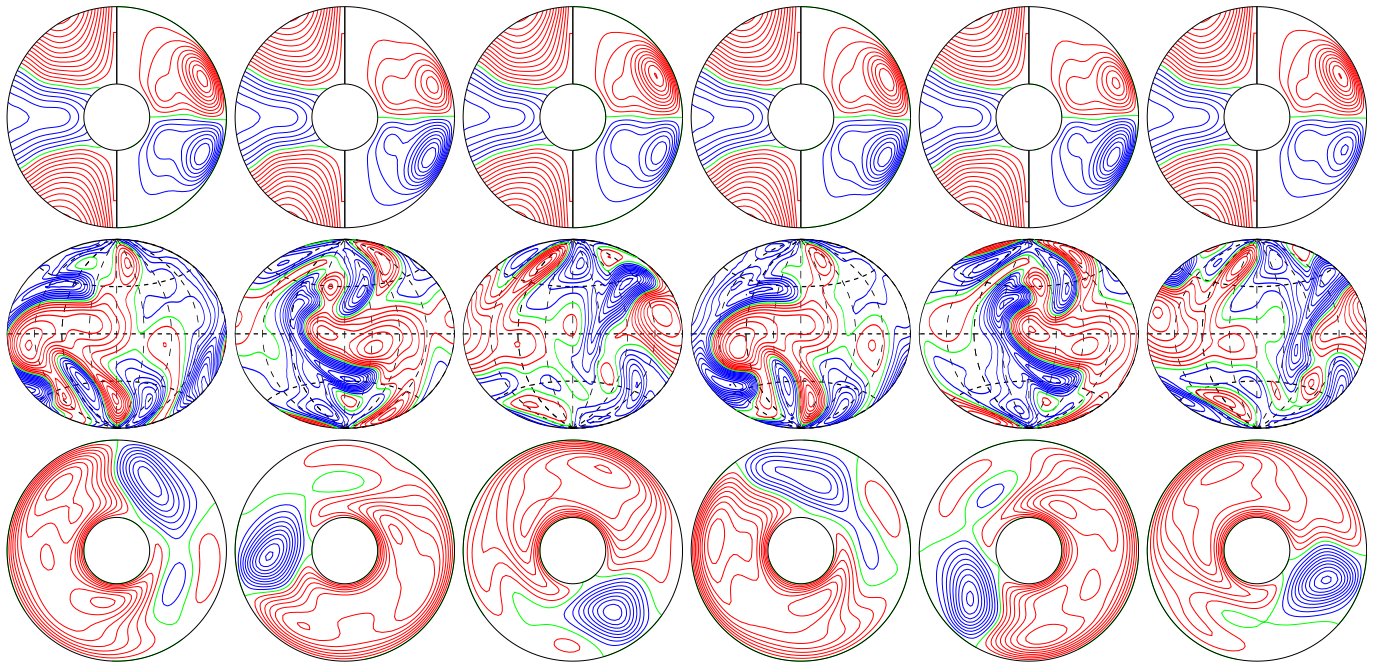
a.e03p1t03r-10m1n2N1z1.224e5 E_{\text{kin}}
