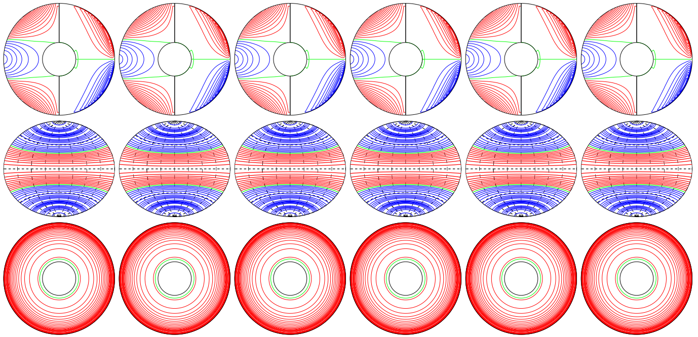
a.e03p1t10r-10m1n2N3z099e7 E_{\text{kin}}
