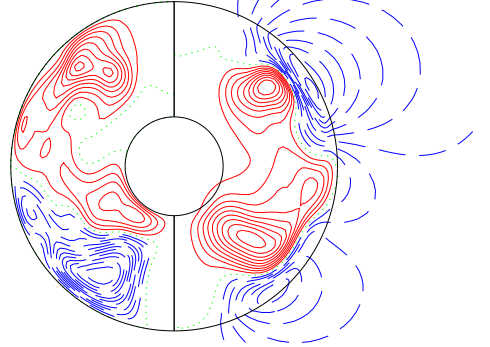
\bar{B}_\phi & pol f-lines (mer)
