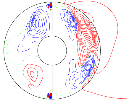
\bar{B}_\phi & pol f-lines (mer)
