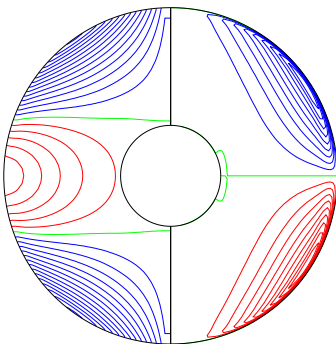
\bar{u}_\phi & merid circulation (mer)
