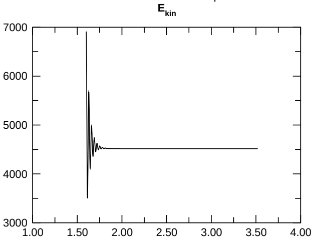
a.e03p1t03r-10m1n2N1z8e4
