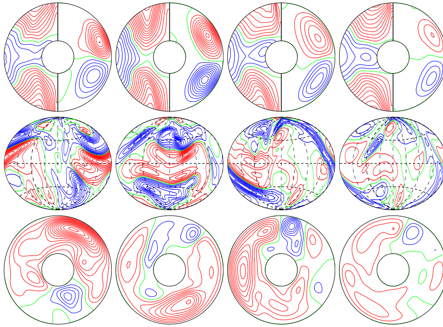
a.e03p1t03r-10m1n2N1z1.45e5 E_{\text{kin}}
