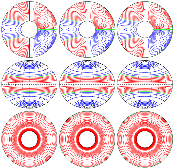
a.e03p1t03r-10m1n2N1z8e4
