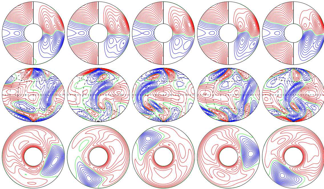
a.e03p1t05r-10m1n2N1z3.03e5 E_{\text{kin}}
