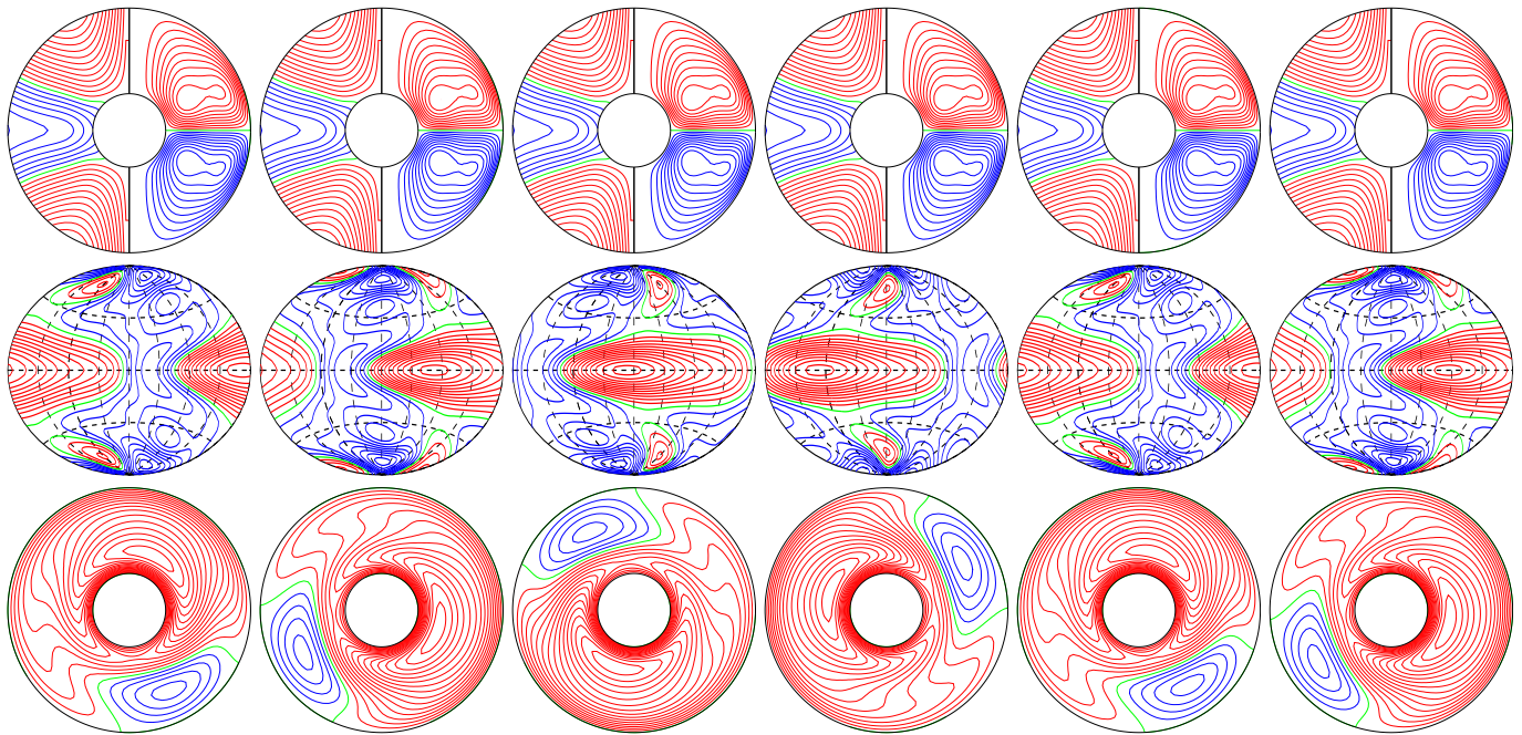
a.e03p1t03r-10m1n2N1z1.15e5 E_{\text{kin}}
