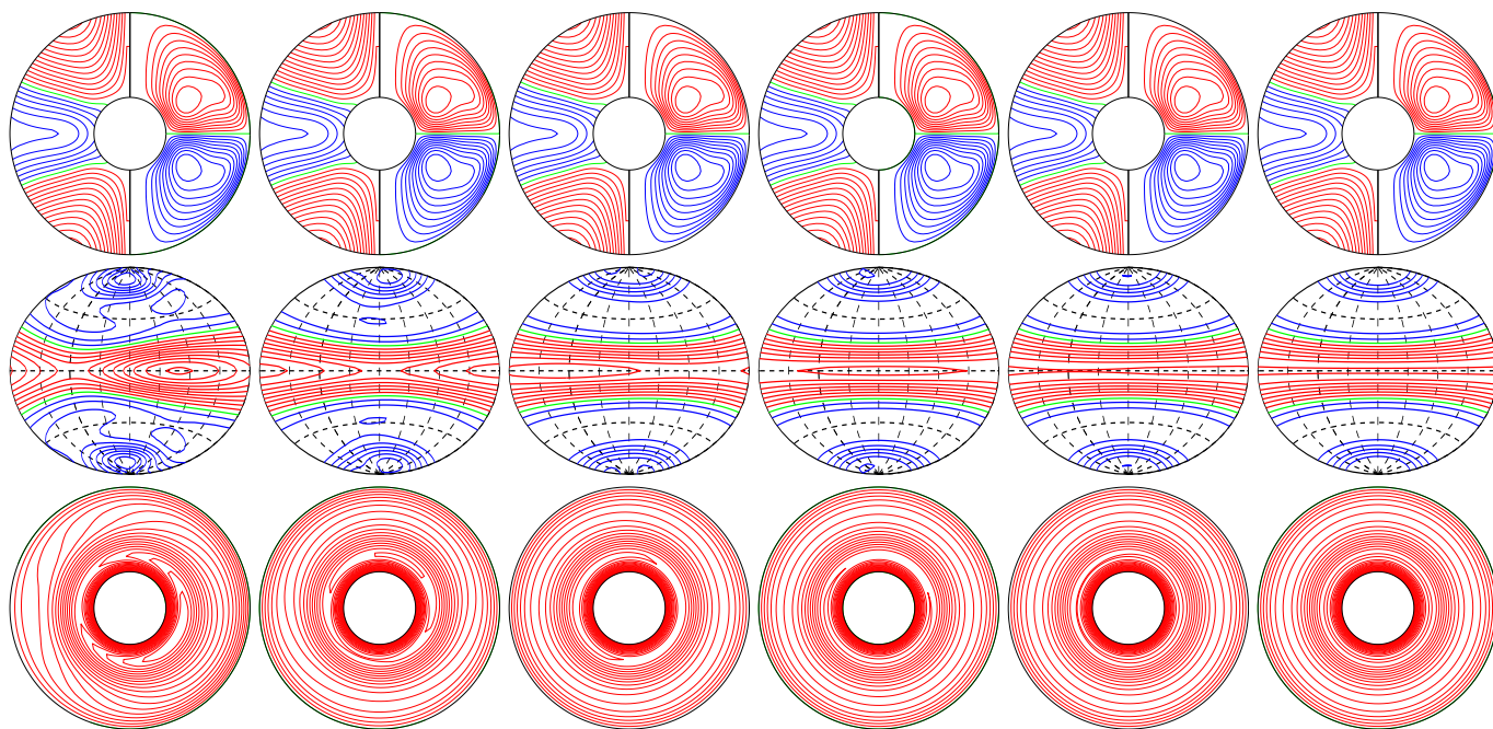
a.e03p1t03r-10m1n2N1z1e5 E_{\text{kin}}
