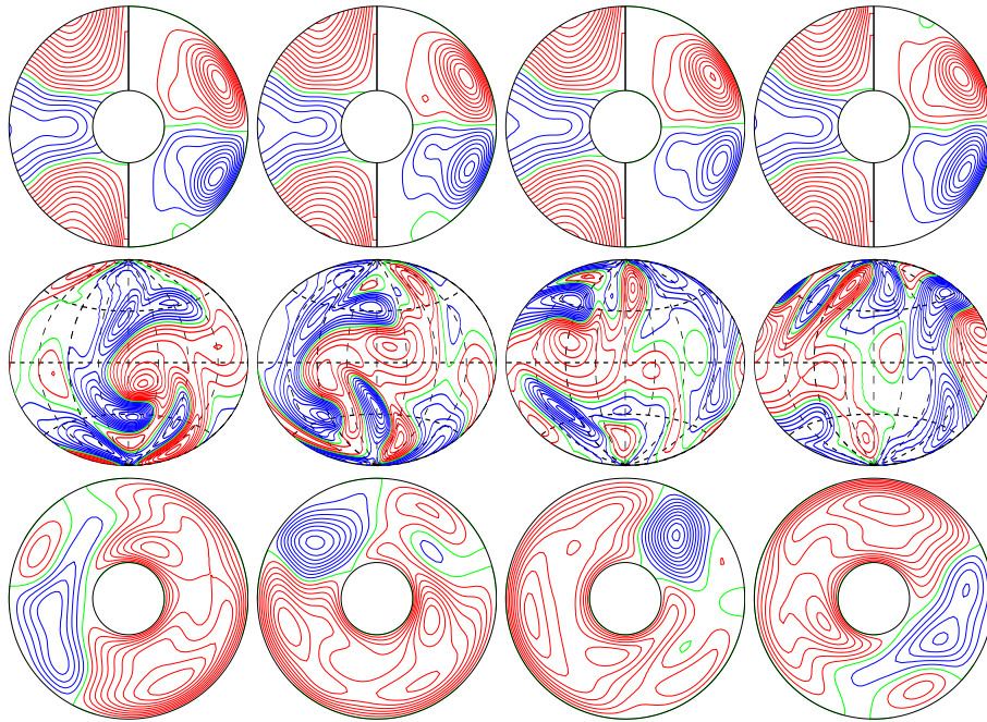
a.e03p1t03r-10m1n2N1z1.27e5 E_{\text{kin}}
