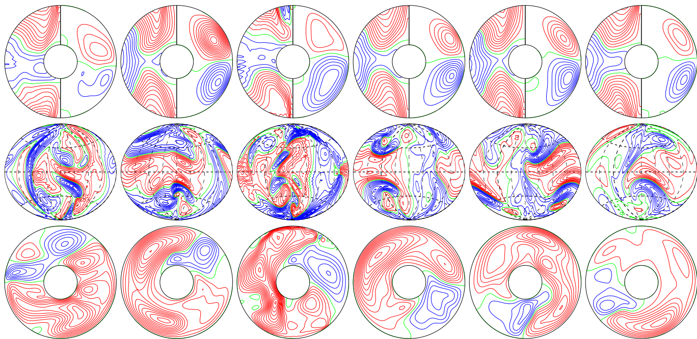
a.e03p1t03r-10m1n2N1z1.5e5 E_{\text{kin}}
