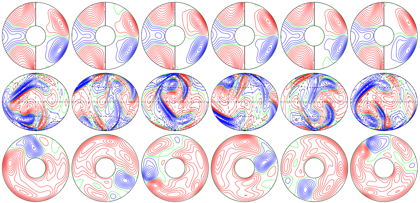
a.e03p1t03r-10m1n2N1z1.39e5 E_{\text{kin}}
