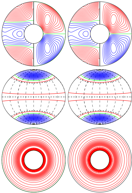
a.e03p1t03r-10m1n2N1z1e2
