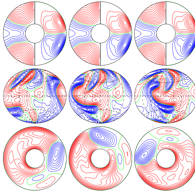
a.e03p1t03r-1000m1n2N1z1.25e5 E_{\text{kin}}
