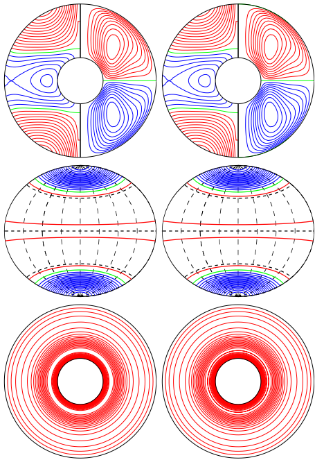
a.e03p1t03r-10m1n2N1z1e1
