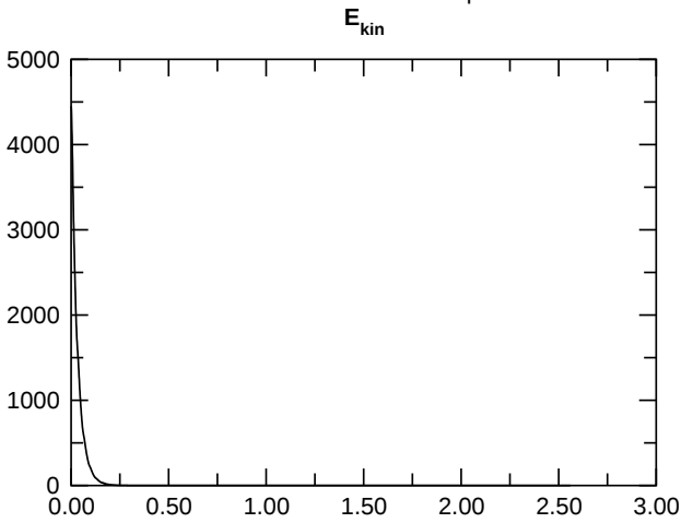
a.e03p1t03r-10m1n2N1z1e1
