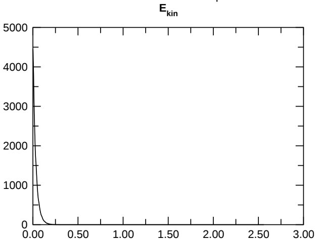
a.e03p1t03r-10m1n2N1z1e2
