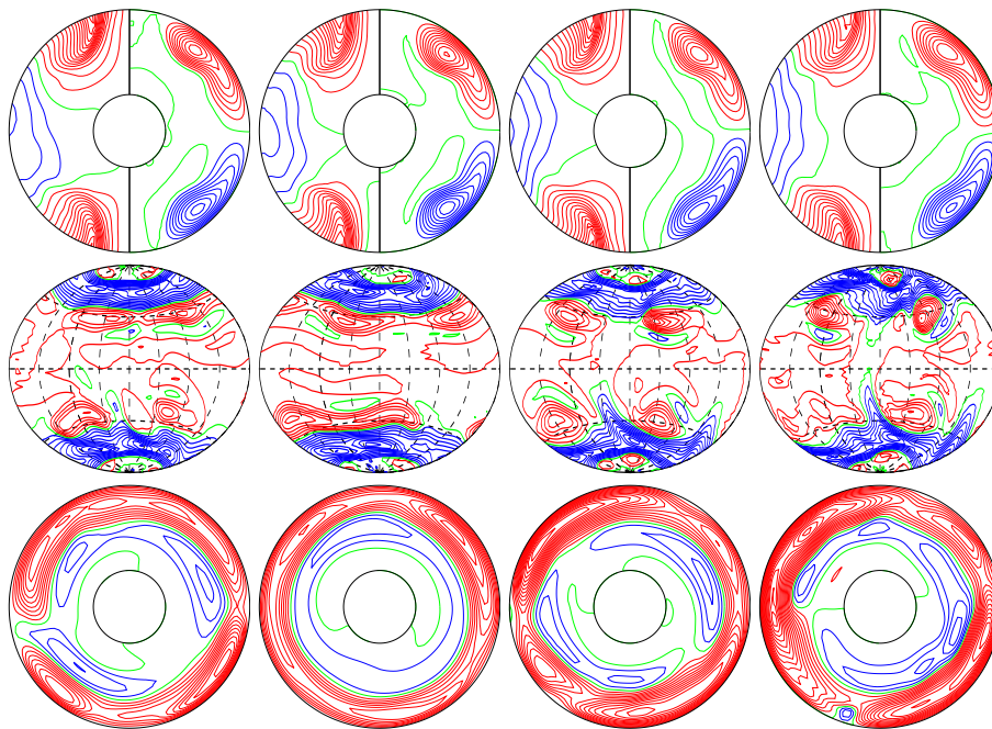
a.e03p1t03r-100000m1p2n2N3z2.5e5 E_{\text{kin}}
