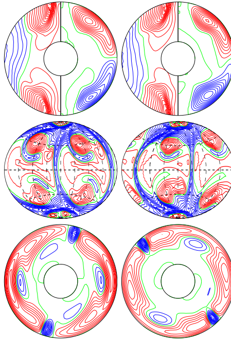
a.e03p1t03r-100000m1n2N3z2.6e5 E_{\text{kin}}
