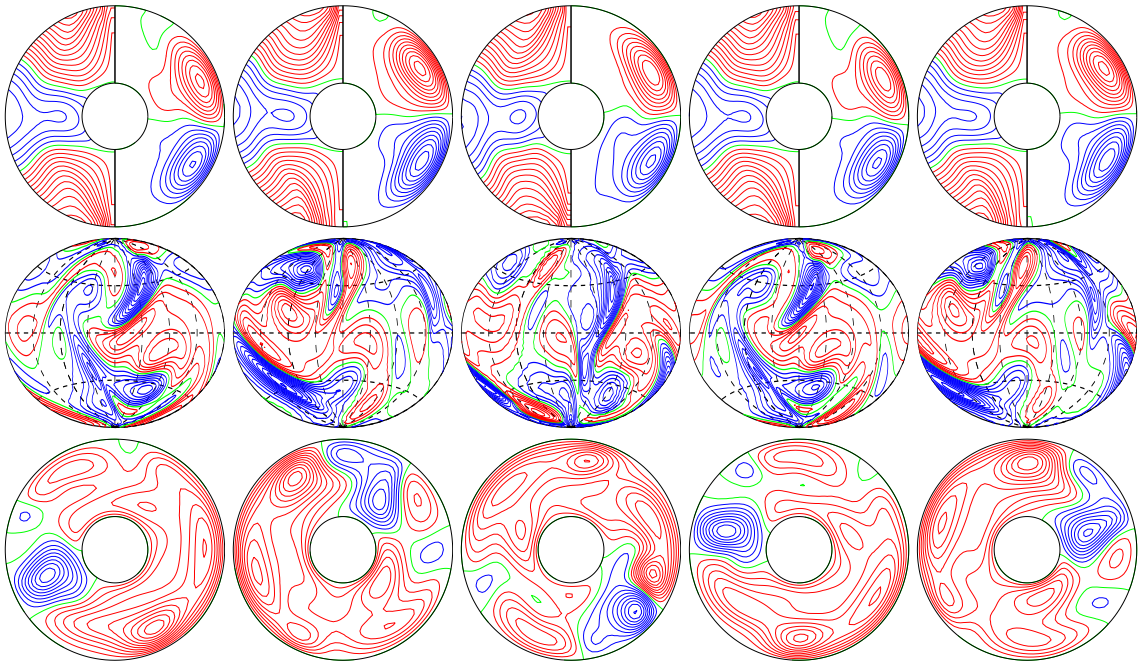
a.e03p1t03r0m1n2N1z1.4e5
