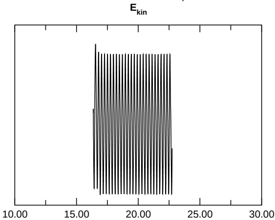
a.e03p1t03r0m1n2N1z1.4e5
