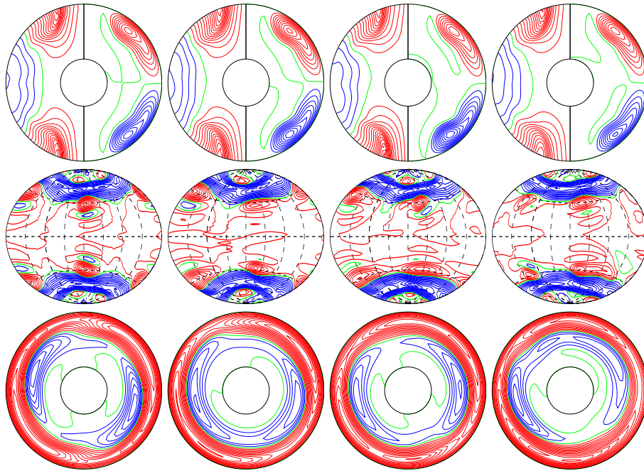
a.e03p1t03r-100000m1p2n2N3z2e5 E_{\text{kin}}
