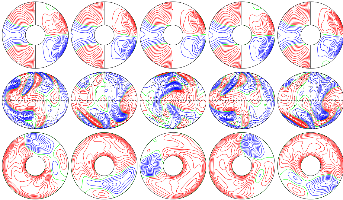
a.e03p1t03r0m1n2N1z1.25e5 E_{\text{kin}}
