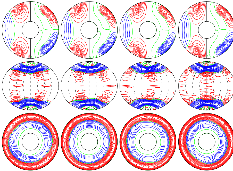
a.e03p1t03r-100000m1p5n2N3z1.5e5 E_{\text{kin}}
