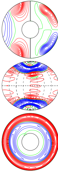
a.e03p1t03r-100000m1p2n2N3z1.8e5 E_{\text{kin}}
