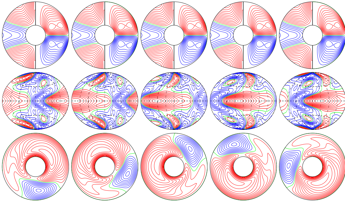
a.e03p1t03r0m1n2N1z1.222e5 E_{\text{kin}}
