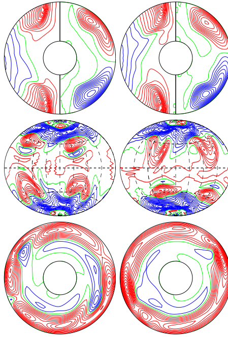
a.e03p1t03r-100000m1p1n2N3z2.8e5 E_{\text{kin}}
