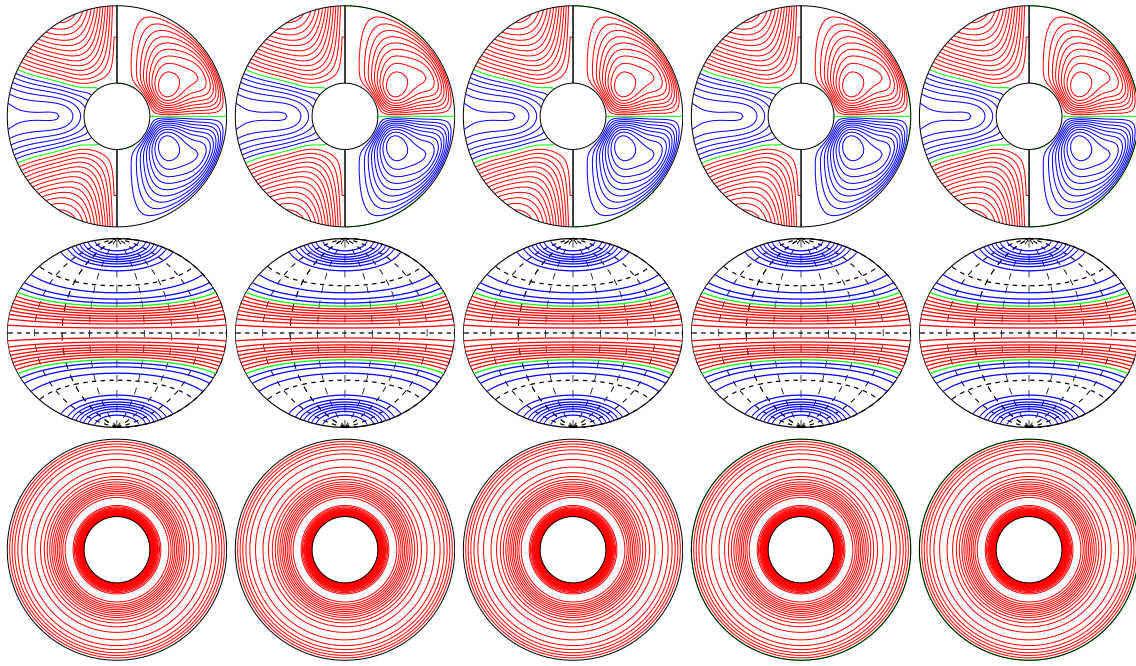
a.e03p1t03r0m1n2N1z9e4 E_{\text{kin}}
