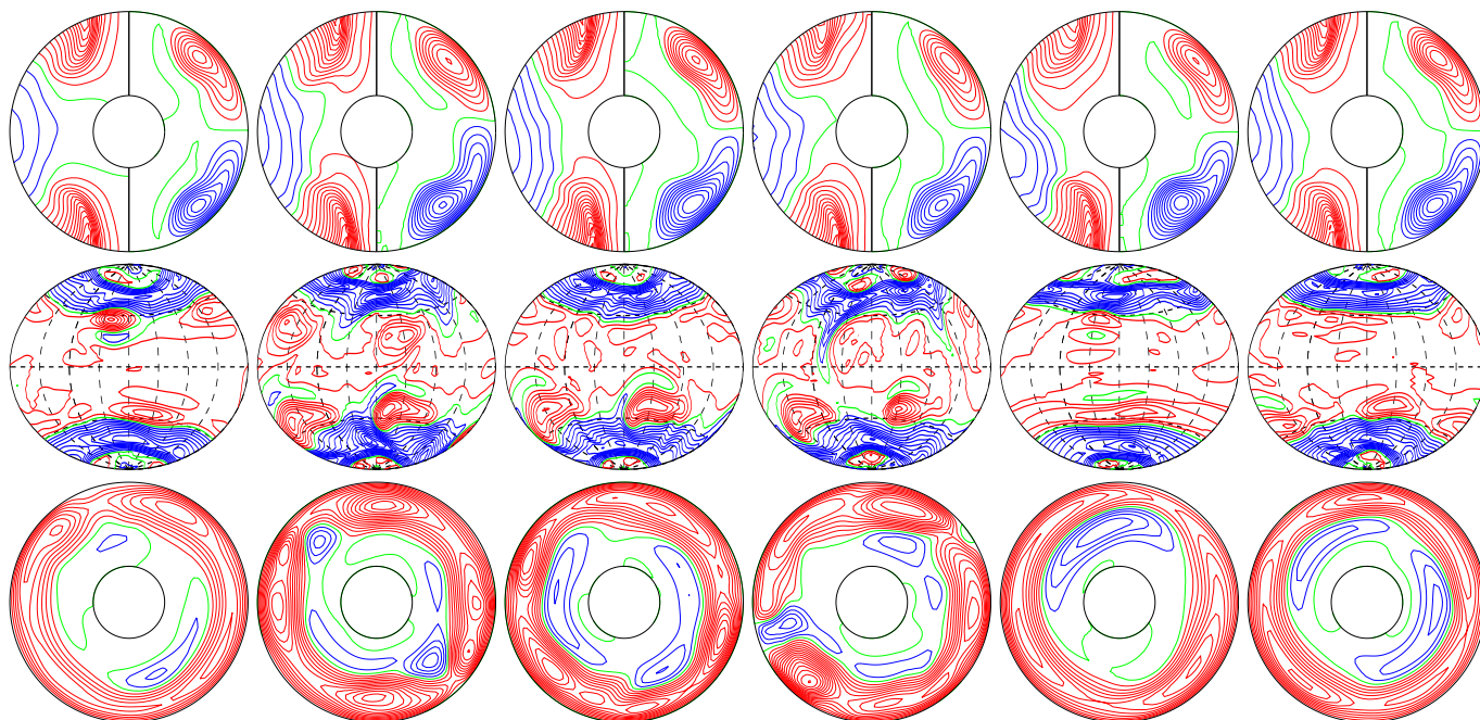
a.e03p1t03r-10m1p2n2N3z1.8e5 E_{\text{kin}}
