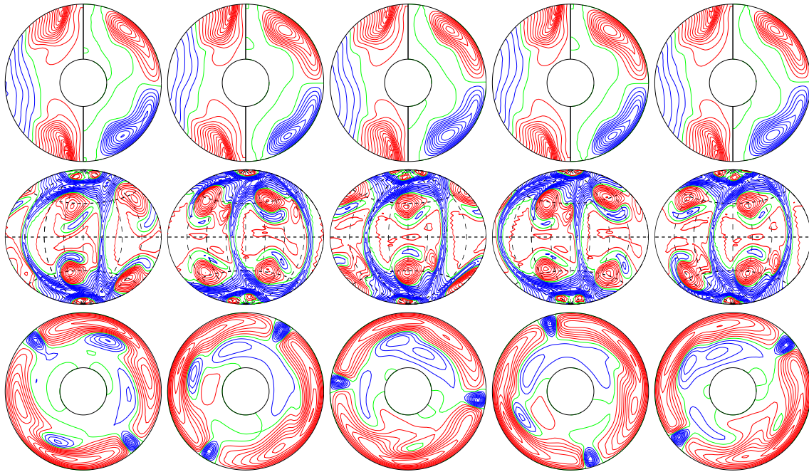
a.e03p1t03r-100000m1n2N3z2.5e5 E_{\text{kin}}
