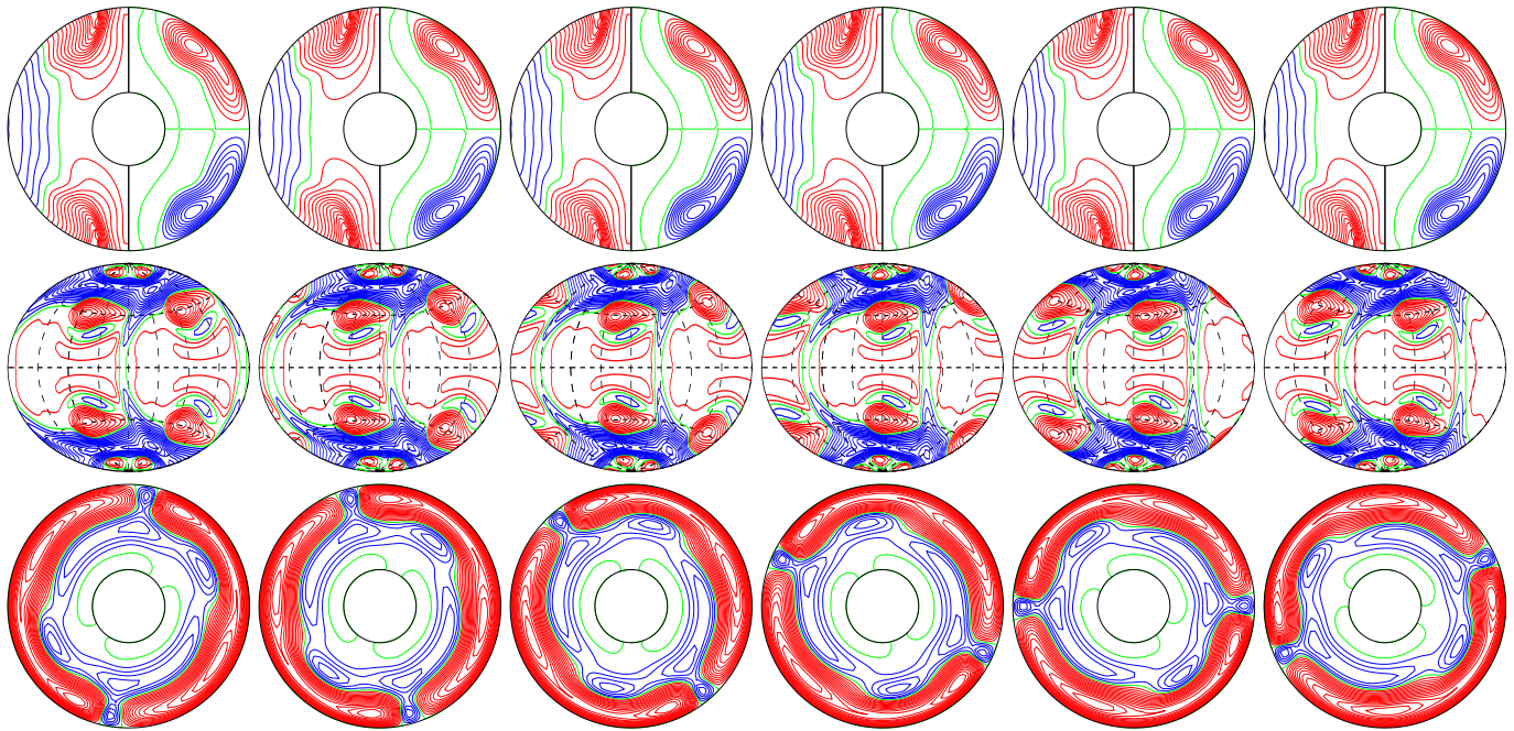
a.e03p1t03r-100000m1n2N3z2e5 E_{\text{kin}}
