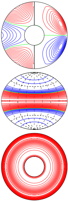
a.e03p1t03r-100000m1n2N1z1.5e5 E_{\text{kin}}
