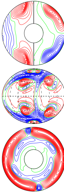
a.e03p1t03r-100000m1n2N3z2.2e5 E_{\text{kin}}
