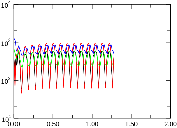
E_{kin,asymm.}
