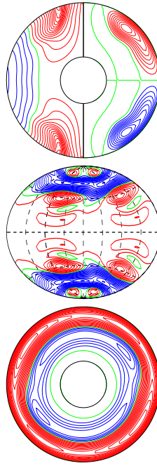
a.e03p1t03r-100000m1n2N3z1.6e5 E_{\text{kin}}
