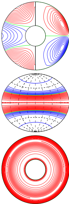
a.e03p1t03r-100000m1n2N1z1.4e5 E_{\text{kin}}
