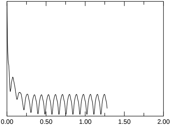
E_{kin,asymm.}
