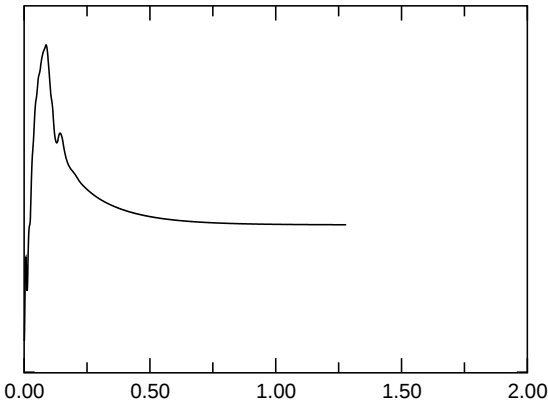
E_{kin,asymm.}
