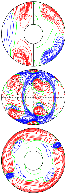
a.e03p1t03r-100000m1n2N3z2.55e5 E_{\text{kin}}
