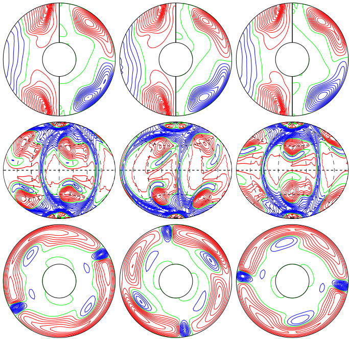
a.e03p1t03r-100000m1n2N3z2.55e5 E_{\text{kin}}
