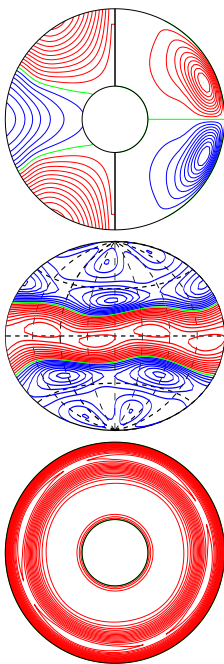
a.e03p1t03r-100000m1n2N1z1.85e5 E_{\text{kin}}
