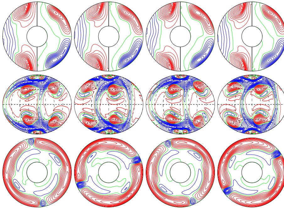
a.e03p1t03r-100000m1n2N3z2.2e5 E_{\text{kin}}
