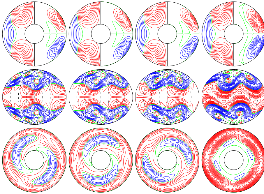
a.e03p1t03r-100000m1n2N1z2e5 E_{\text{kin}}
