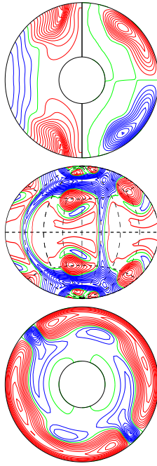
a.e03p1t03r-100000m1n2N3z2.1e5 E_{\text{kin}}
