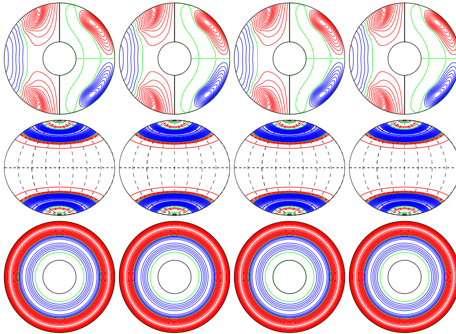
a.e03p1t03r-100000m1n2N3z1.3e5 E_{\text{kin}}
