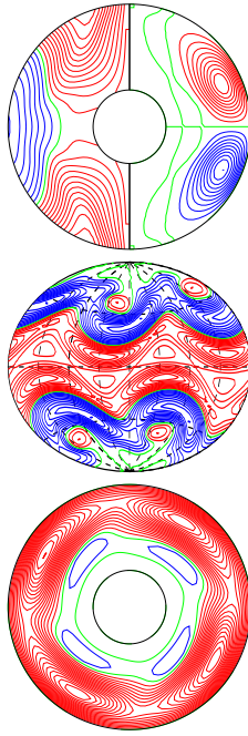
a.e03p1t03r-100000m1n2N1z2.1e5 E_{\text{kin}}
