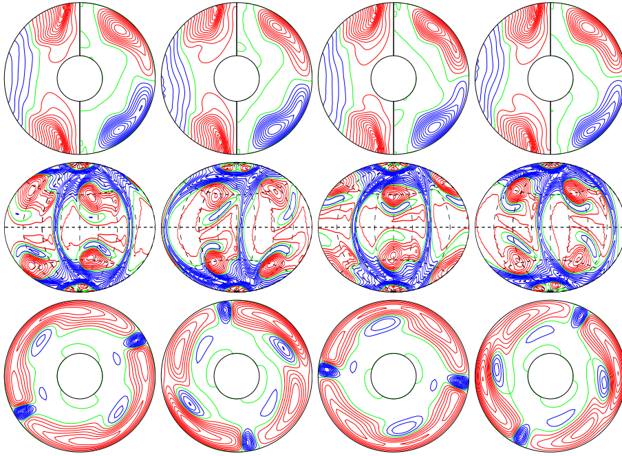
a.e03p1t03r-100000m1n2N3z2.55e5 E_{\text{kin}}
