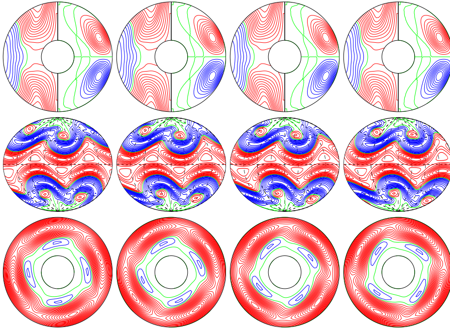
a.e03p1t03r-100000m1n2N1z2.2e5 E_{\text{kin}}
