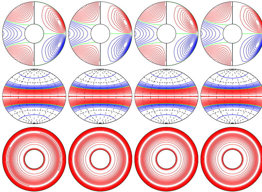
a.e03p1t03r-100000m1n2N1z1.4e5 E_{\text{kin}}
