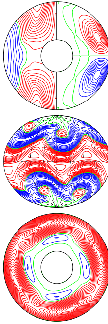
a.e03p1t03r-100000m1n2N1z2.15e5 E_{\text{kin}}
