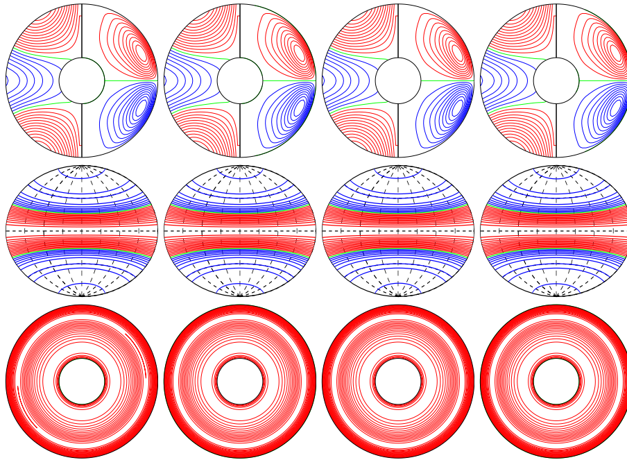
a.e03p1t03r-100000m1n2N1z1.3e5 E_{\text{kin}}
