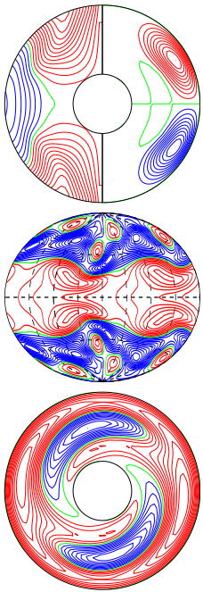
a.e03p1t03r-100000m1n2N1z1.95e5 E_{kin}
