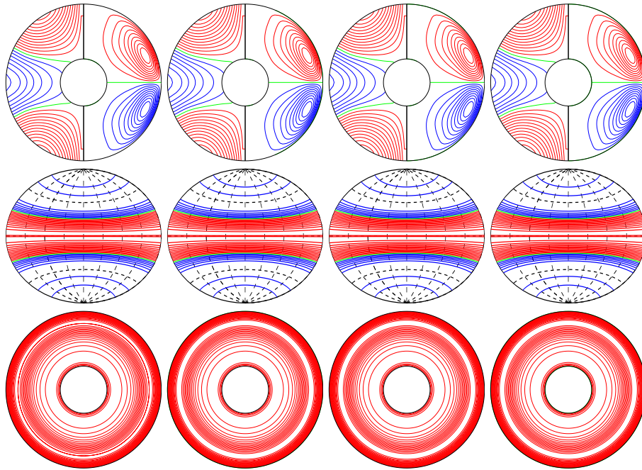
a.e03p1t03r-100000m1n2N1z1.5e5 E_{\text{kin}}
