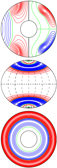
a.e03p1t03r-100000m1n2N3z1.333e5 E_{\text{kin}}
