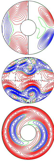
a.e03p1t03r-100000m1n2N1z2.05e5 E_{\text{kin}}
