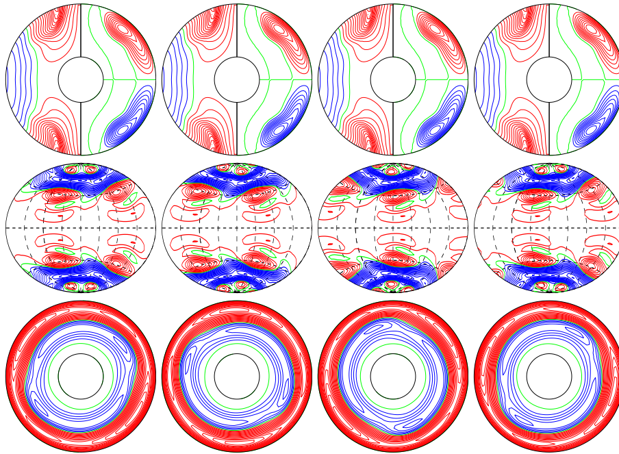
a.e03p1t03r-100000m1n2N3z1.6e5 E_{\text{kin}}
