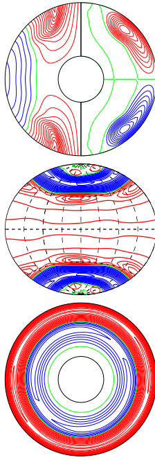
a.e03p1t03r-100000m1n2N3z1.366e5 E_{\text{kin}}
