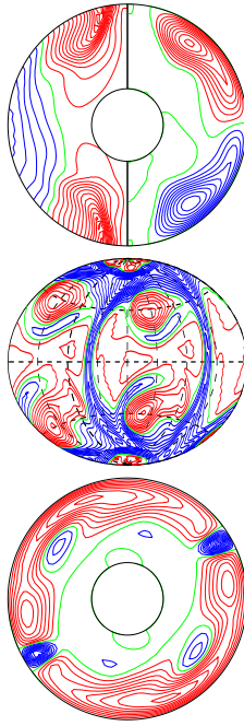
a.e03p1t03r-100000m1n2N3z2.6e5 E_{\text{kin}}
