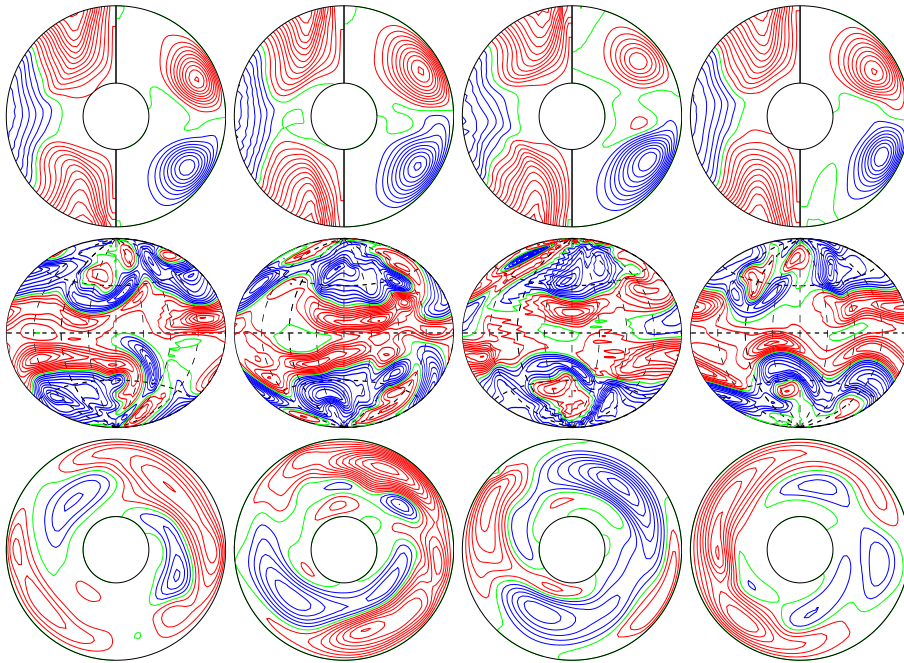
a.e03p1t03r-100000m1n2N1z2.55e5 E_{\text{kin}}
