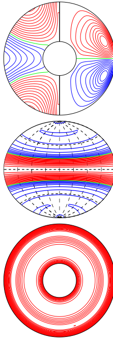
a.e03p1t03r-30000m1n2N1z1.5e5 E_{\text{kin}}
