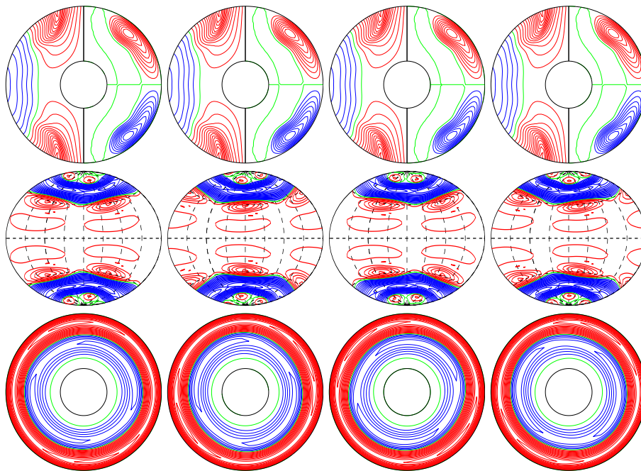
a.e03p1t03r-100000m1n2N3z1.4e5 E_{\text{kin}}
