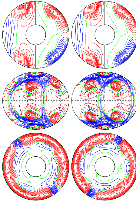
a.e03p1t03r-100000m1n2N3z2.15e5 E_{\text{kin}}
