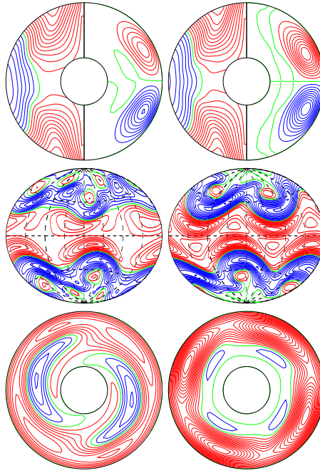
a.e03p1t03r-100000m1n2N1z2.05e5 E_{\text{kin}}
