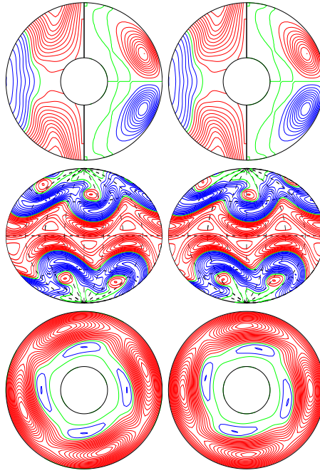
a.e03p1t03r-100000m1n2N1z2.15e5 E_{\text{kin}}
