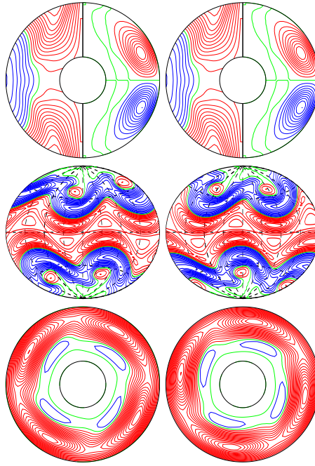
a.e03p1t03r-100000m1n2N1z2.1e5 E_{\text{kin}}
