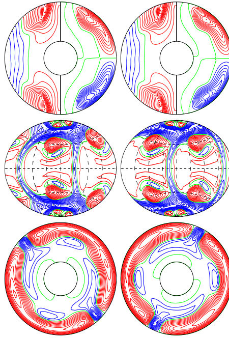
a.e03p1t03r-100000m1n2N3z2.1e5 E_{\text{kin}}
