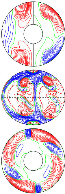
a.e03p1t03r-100000m1n2N3z2.58e5 E_{\text{kin}}
