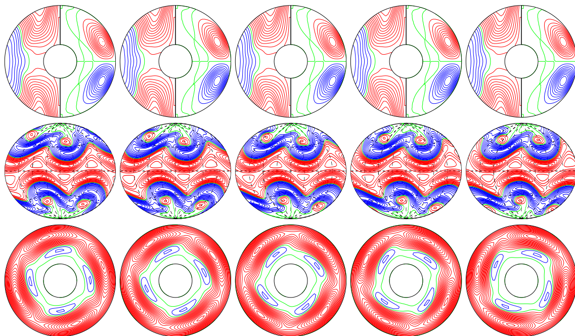
a.e03p1t03r-100000m1n2N1z2.2e5 E_{\text{kin}}
