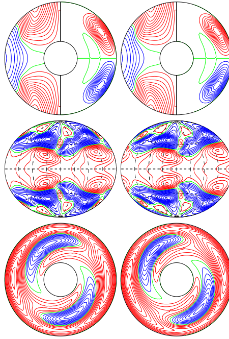
a.e03p1t03r-100000m1n2N1z1.9e5 E_{\text{kin}}
