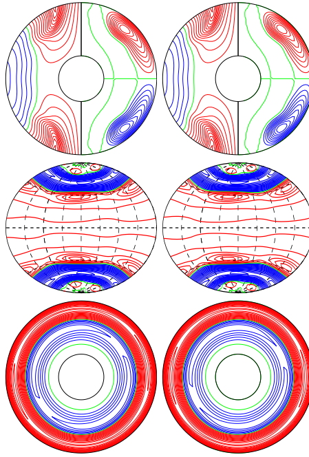
a.e03p1t03r-100000m1n2N3z1.366e5 E_{\text{kin}}
