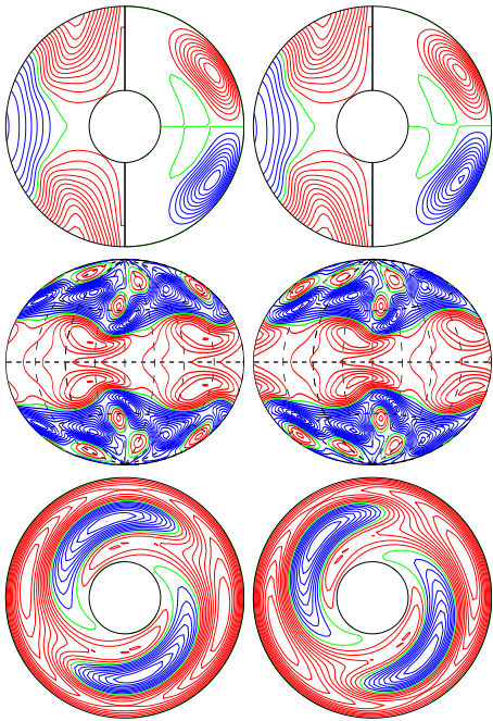
a.e03p1t03r-100000m1n2N1z1.95e5 E_{\text{kin}}
