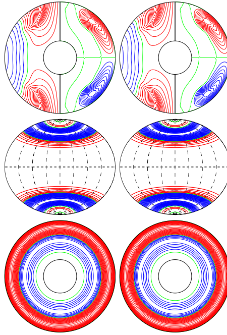
a.e03p1t03r-100000m1n2N3z1.333e5 E_{\text{kin}}
