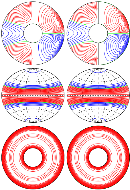
a.e03p1t03r-30000m1n2N1z1.3e5 E_{\text{kin}}
