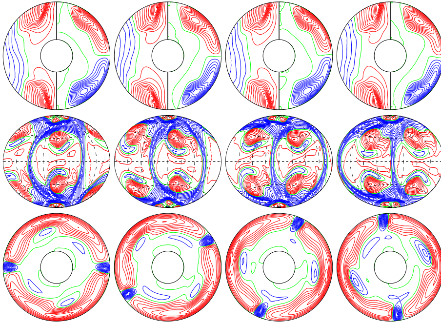
a.e03p1t03r-100000m1n2N3z2.52e5 E_{\text{kin}}
