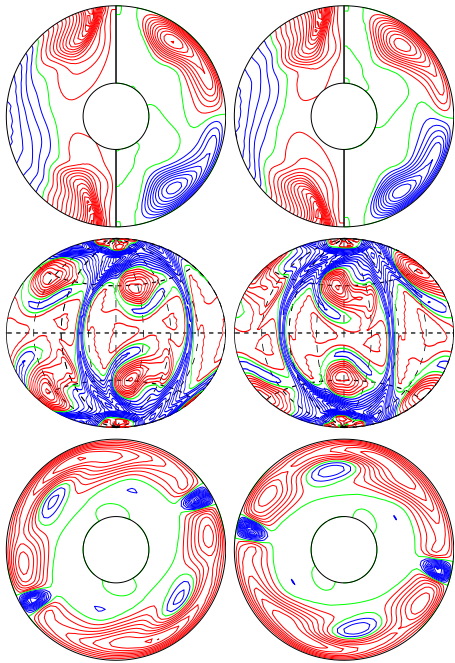
a.e03p1t03r-100000m1n2N3z2.6e5 E_{\text{kin}}
