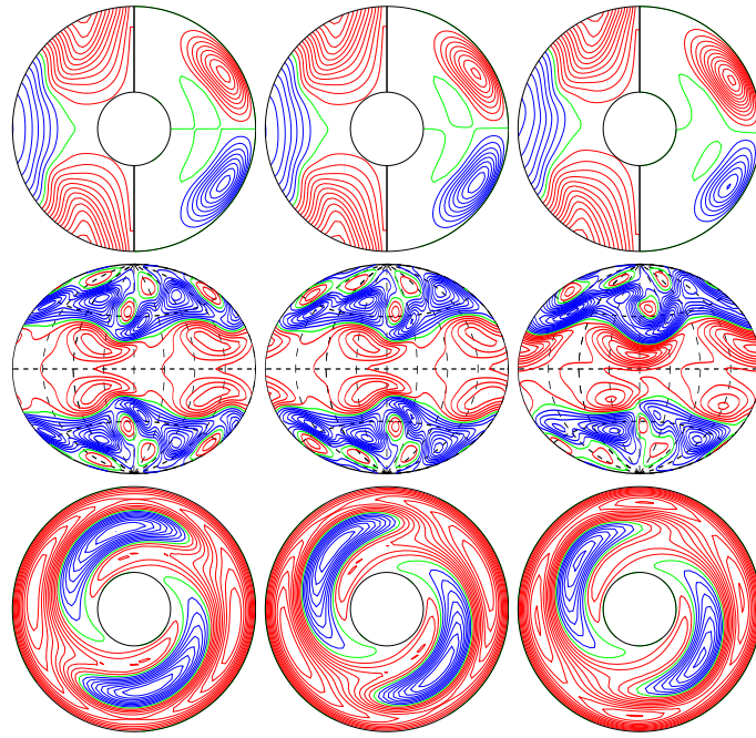
a.e03p1t03r-100000m1n2N1z1.95e5 E_{kin}
