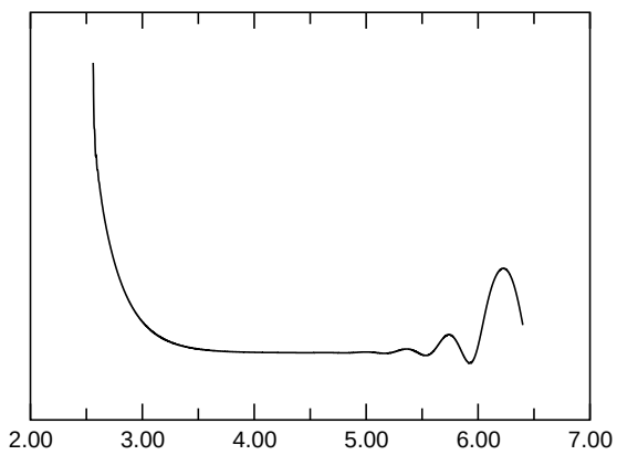
E_{kin,asymm.}
