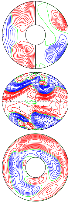
a.e03p1t03r-100000m1n2N1z2.504e5 E_{\text{kin}}
