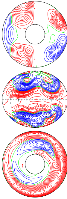
a.e03p1t03r-100000m1n2N1z2.503e5 E_{\text{kin}}
