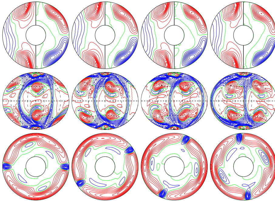
a.e03p1t03r-100000m1n2N3z2.52e5 E_{\text{kin}}
