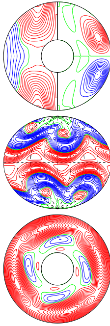
a.e03p1t03r-100000m1n2N1z2.501e5 E_{\text{kin}}
