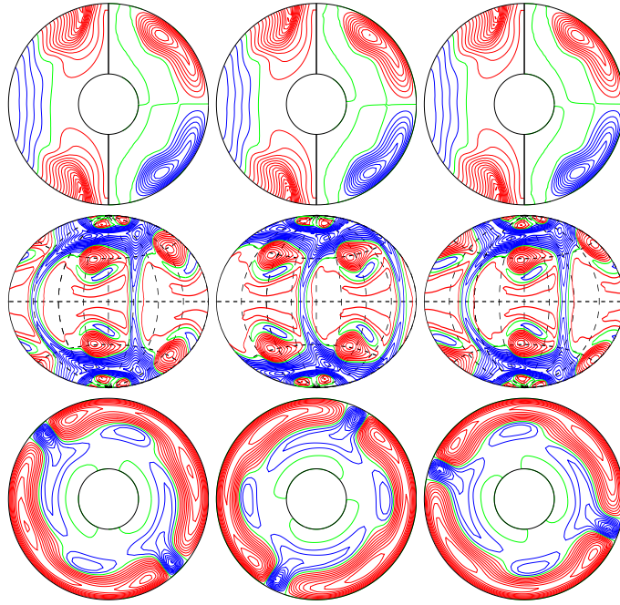
a.e03p1t03r-100000m1n2N3z2.1e5 E_{\text{kin}}
