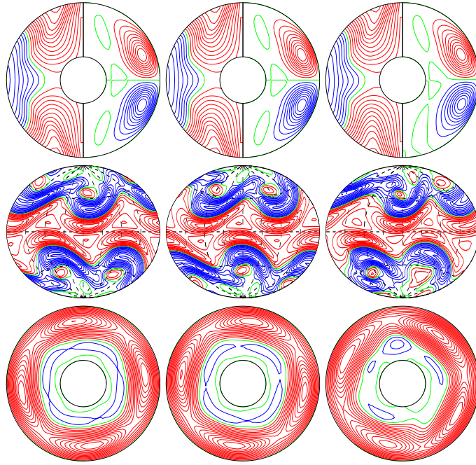
a.e03p1t03r-30000m1n2N1z1.9e5 E_{\text{kin}}
