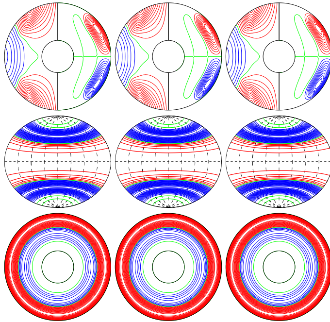
a.e03p1t03r-100000m1n2N3z1.1e5 E_{\text{kin}}
