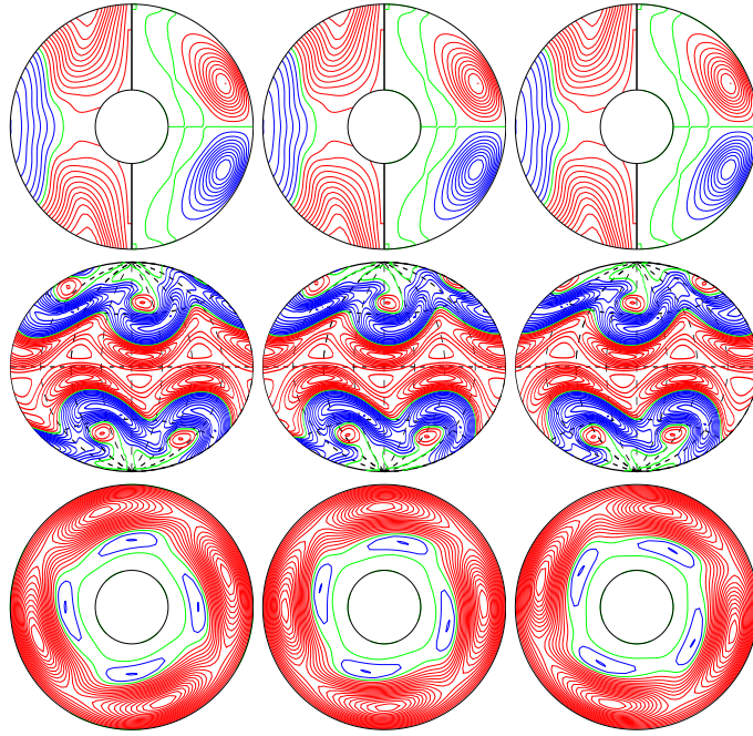
a.e03p1t03r-100000m1n2N1z2.15e5 E_{\text{kin}}
