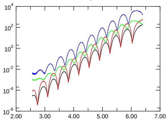
E_{kin,asymm.}
