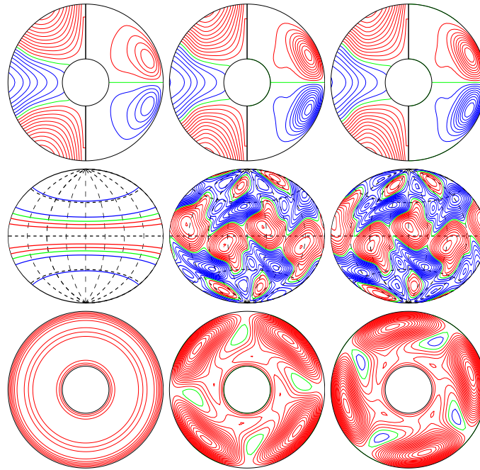
a.e03p1t03r-30000m1n2N1z1.6e5 E_{\text{kin}}
