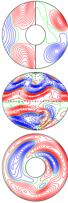
a.e03p1t03r-100000m1n2N1z2.502e5 E_{\text{kin}}
