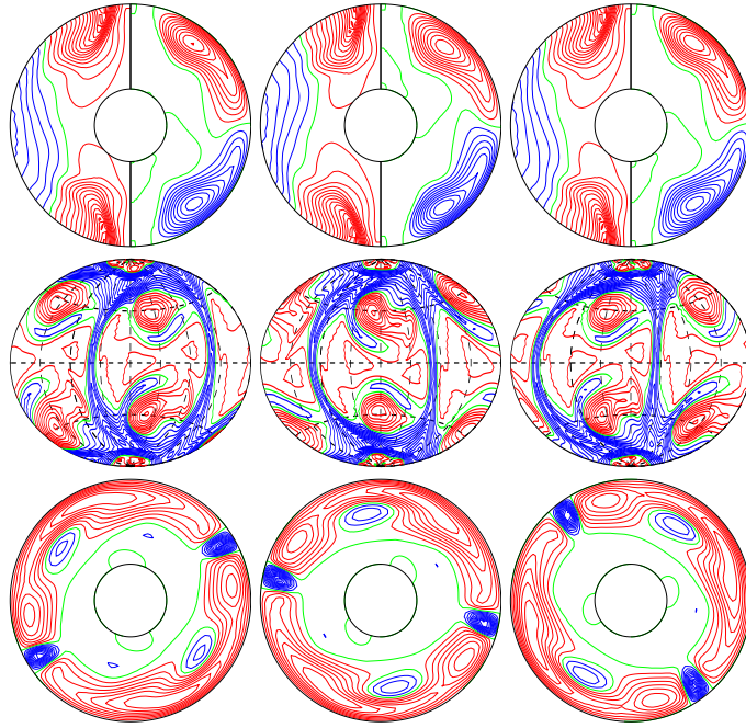
a.e03p1t03r-100000m1n2N3z2.6e5 E_{\text{kin}}
