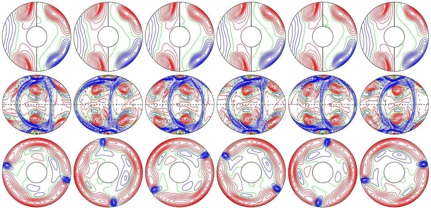
a.e03p1t03r-100000m1n2N3z2.5e5 E_{\text{kin}}
