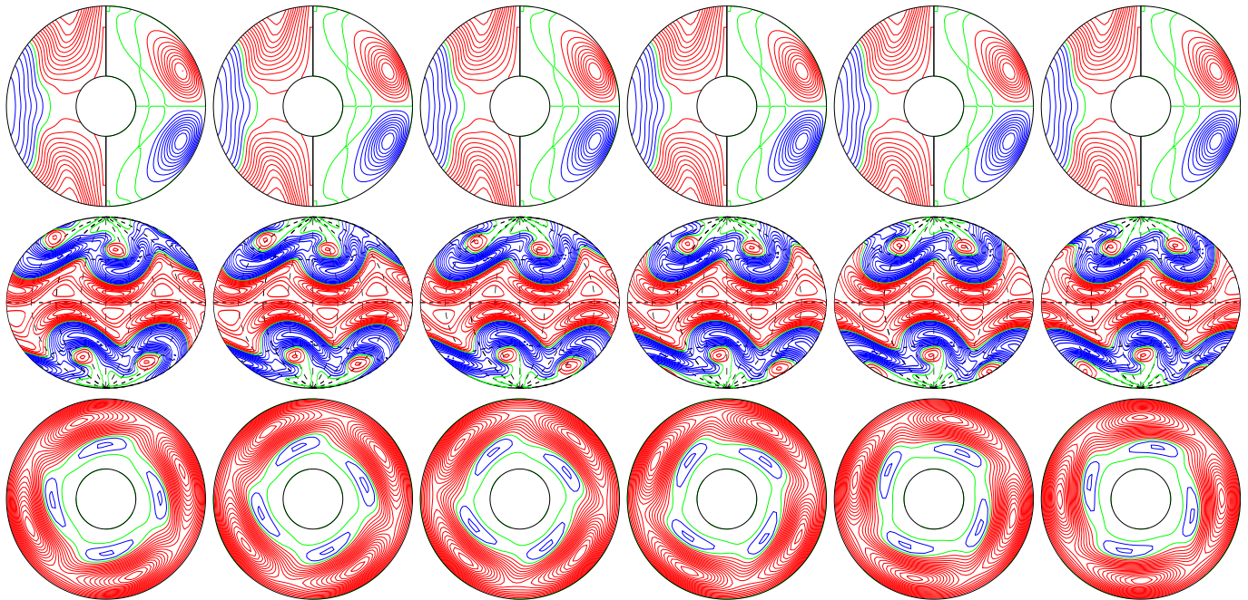
a.e03p1t03r-100000m1n2N1z2.2e5 E_{\text{kin}}
