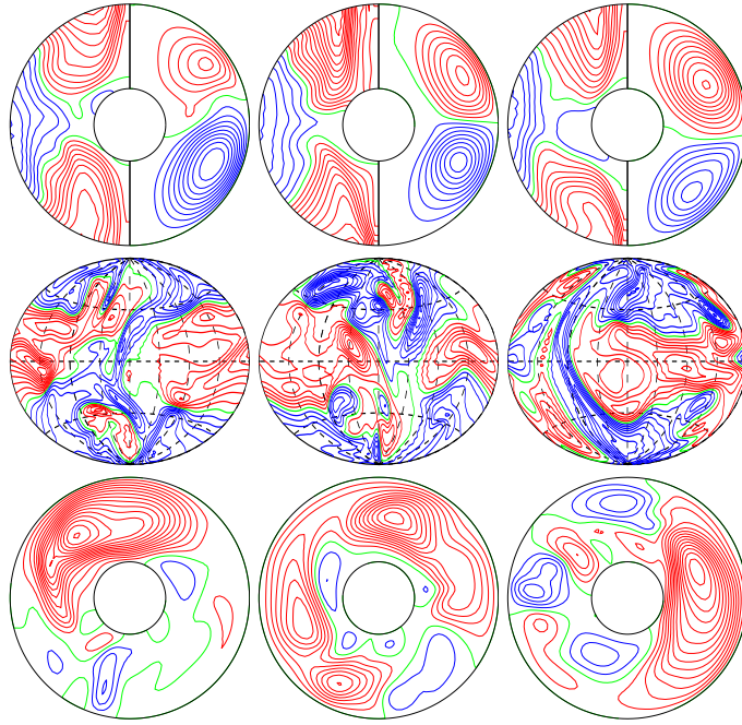
a.e03p1t03r-30000m1n2N1z2.2e5 E_{\text{kin}}
