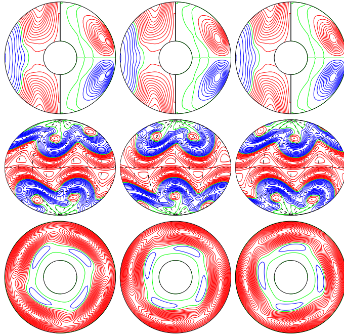
a.e03p1t03r-100000m1n2N1z2.1e5 E_{\text{kin}}
