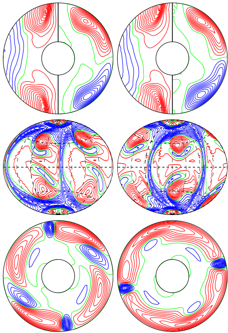
a.e03p1t03r-100000m1n2N3z2.58e5 E_{\text{kin}}
