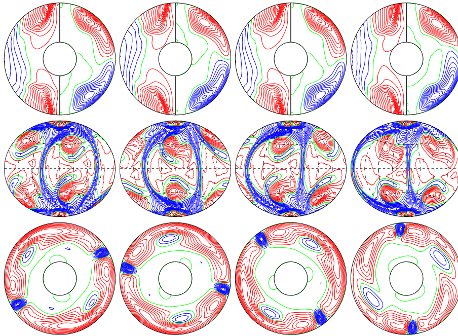
a.e03p1t03r-100000m1n2N3z2.6e5 E_{\text{kin}}
