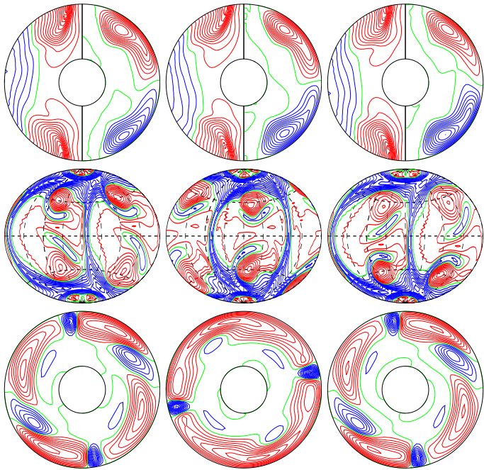
a.e03p1t03r-100000m1n2N3z2.58e5 E_{\text{kin}}
