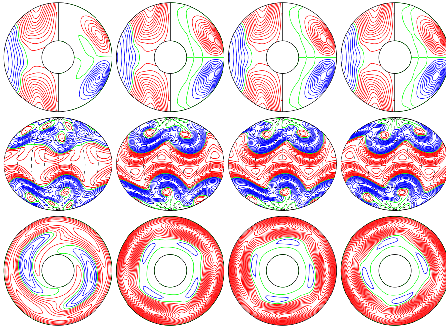
a.e03p1t03r-100000m1n2N1z2.05e5 E_{\text{kin}}
