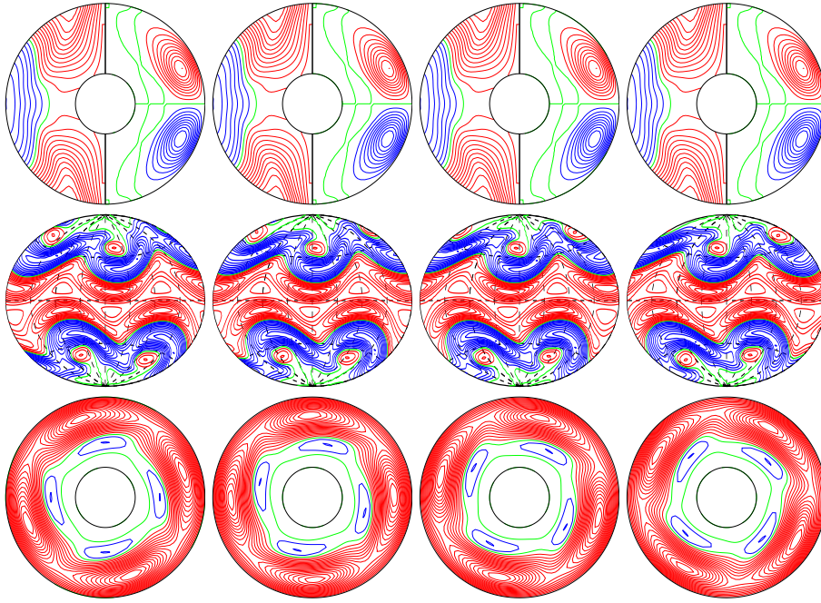
a.e03p1t03r-100000m1n2N1z2.15e5 E_{\text{kin}}
