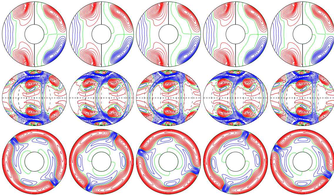
a.e03p1t03r-100000m1n2N3z2.1e5 E_{\text{kin}}
