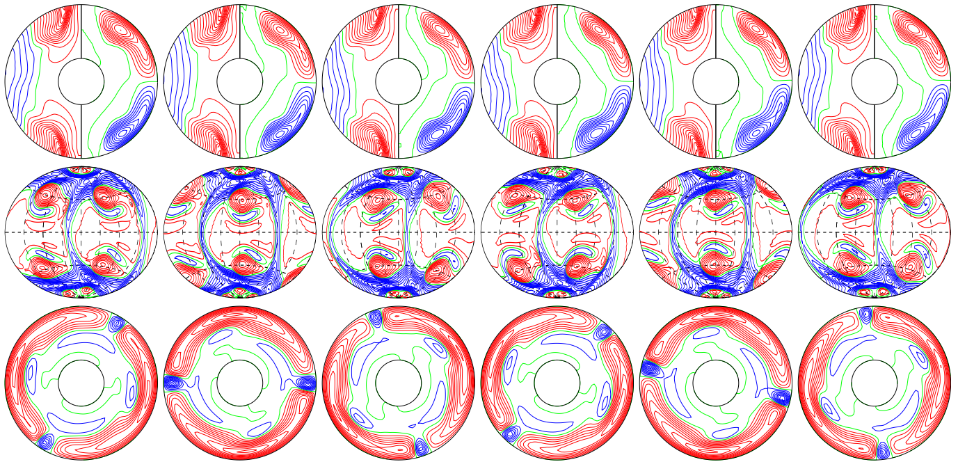
a.e03p1t03r-100000m1n2N3z2.25e5 E_{\text{kin}}
