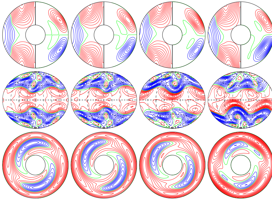
a.e03p1t03r-100000m1n2N1z1.95e5 E_{\text{kin}}
