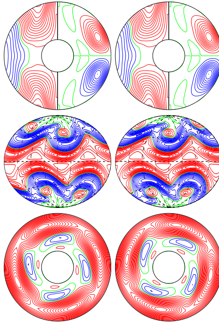
a.e03p1t03r-100000m1n2N1z2.501e5 E_{\text{kin}}
