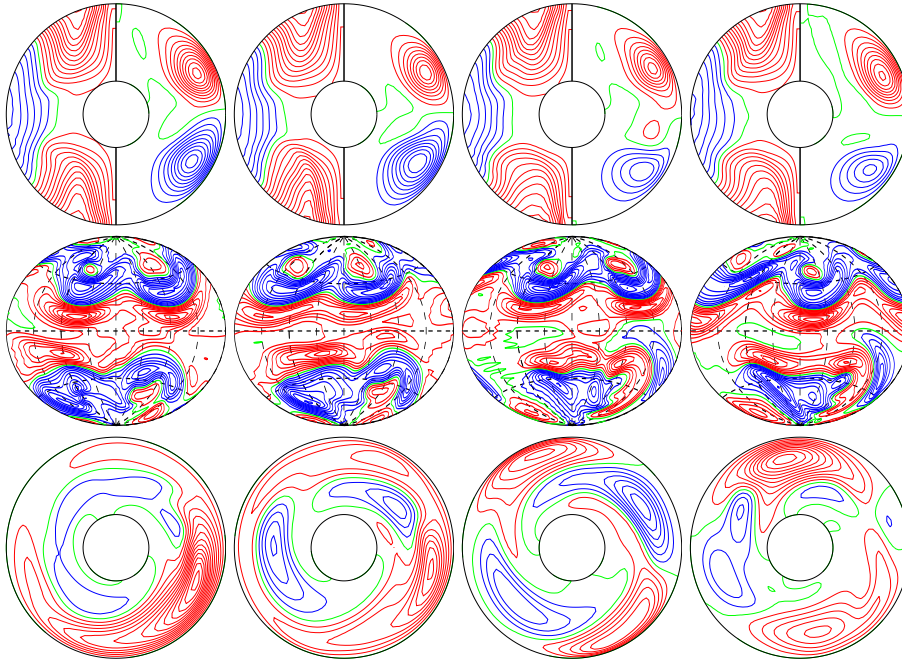
a.e03p1t03r-100000m1n2N1z2.505e5 E_{\text{kin}}
