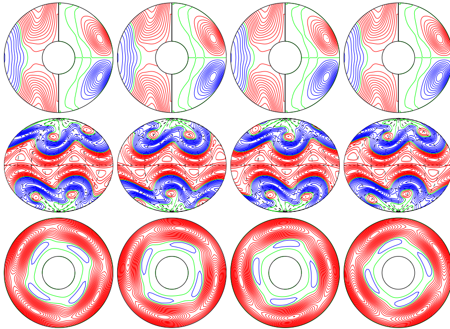
a.e03p1t03r-100000m1n2N1z2.1e5 E_{\text{kin}}
