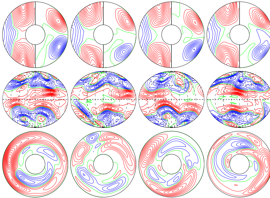
a.e03p1t03r-100000m1n2N1z2.515e5 E_{\text{kin}}
