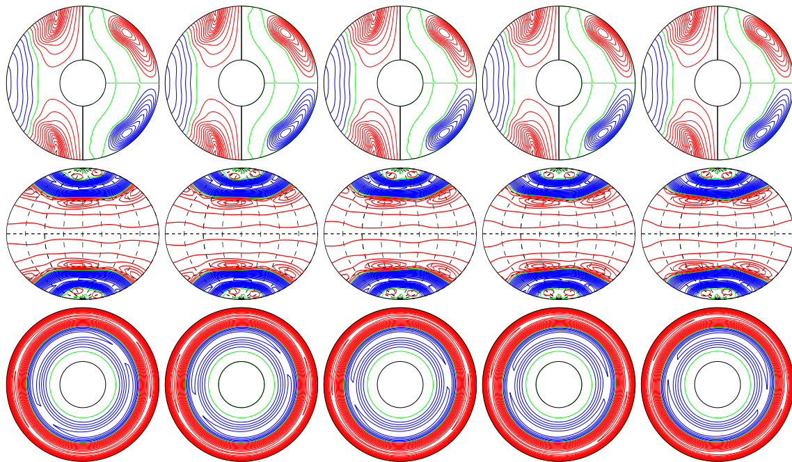
a.e03p1t03r-100000m1n2N3z1.366e5 E_{\text{kin}}
