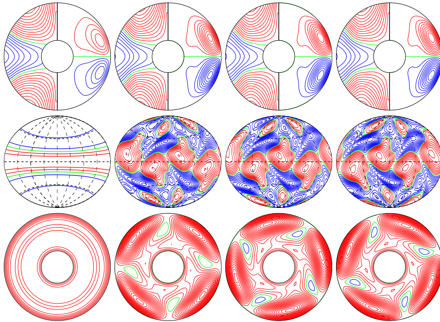
a.e03p1t03r-30000m1n2N1z1.6e5 E_{\text{kin}}
