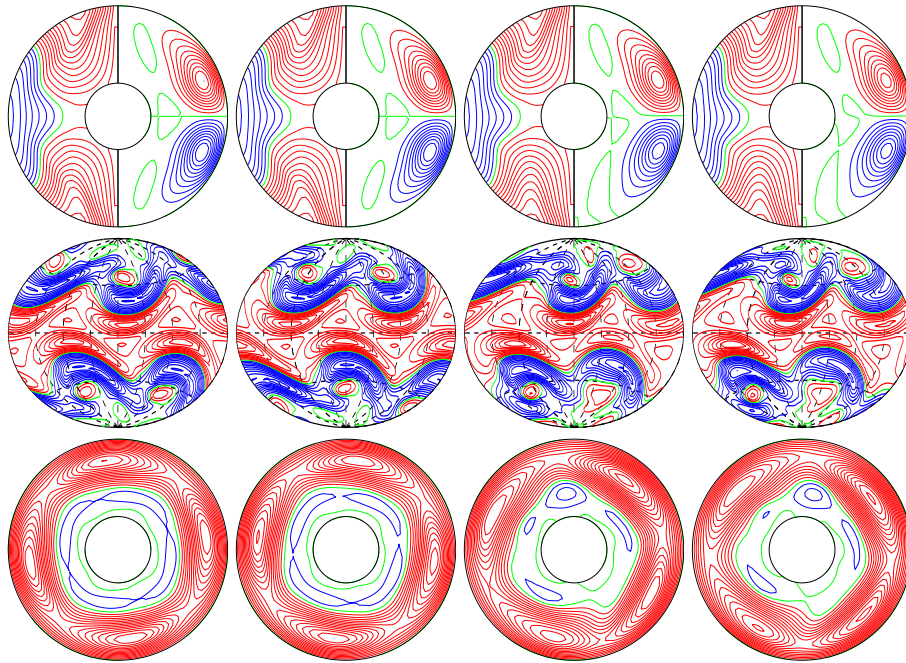
a.e03p1t03r-30000m1n2N1z1.9e5 E_{\text{kin}}
