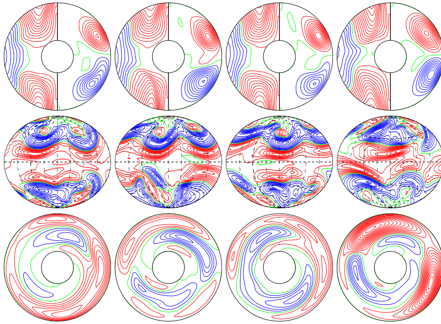
a.e03p1t03r-100000m1n2N1z2.503e5 E_{\text{kin}}
