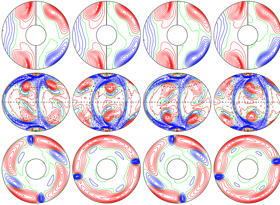
a.e03p1t03r-100000m1n2N3z2.58e5 E_{\text{kin}}
