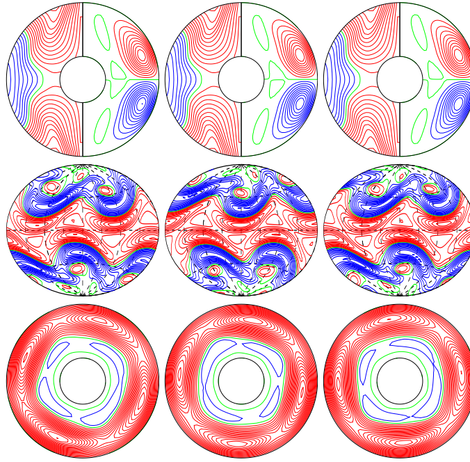
a.e03p1t03r-30000m1n2N1z1.8e5 E_{\text{kin}}
