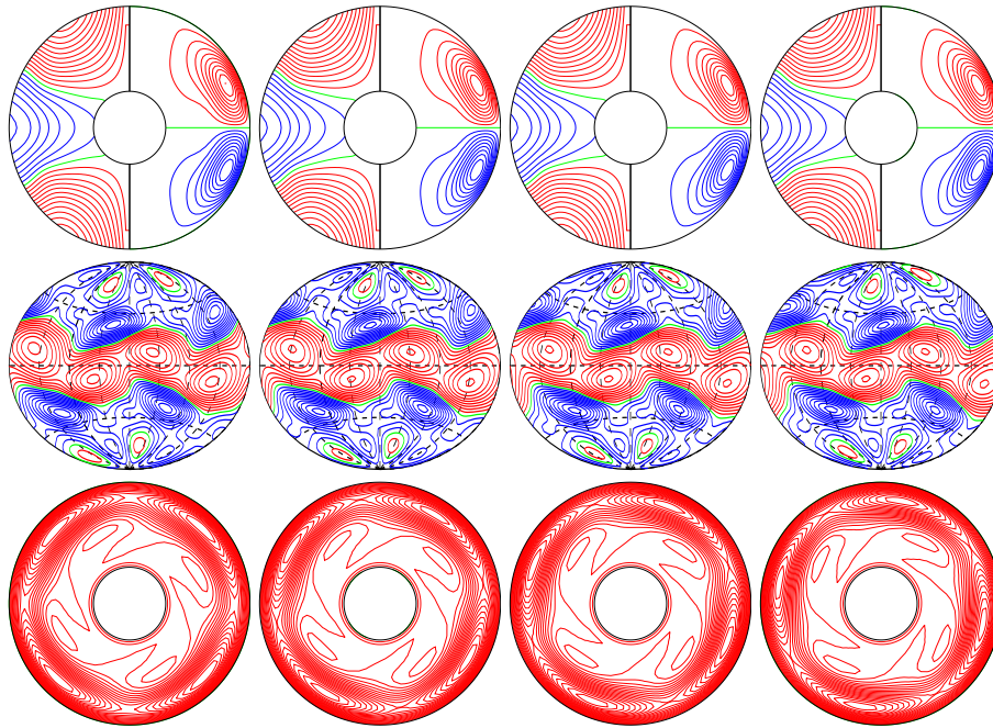
a.e03p1t03r-100000m1n2N1z1.8e5 E_{\text{kin}}
