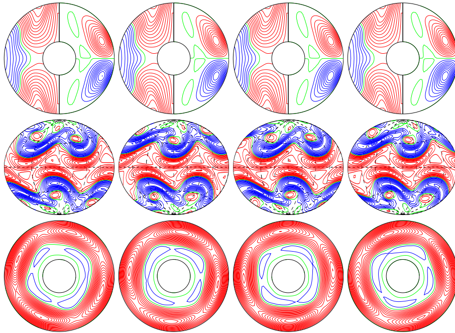
a.e03p1t03r-30000m1n2N1z1.8e5 E_{\text{kin}}
