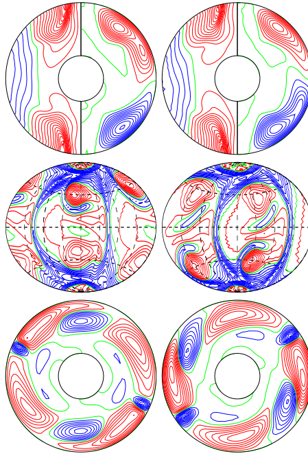
a.e03p1t03r-100000m1n2N3z2.595e5 E_{\text{kin}}
