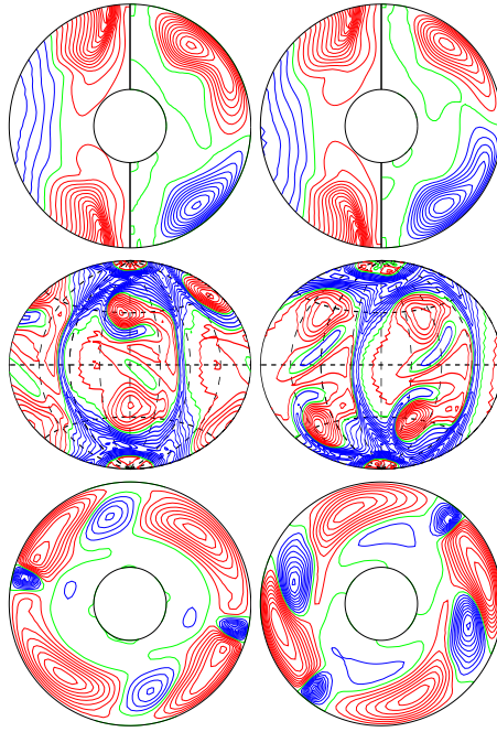
a.e03p1t03r-100000m1n2N3z2.59e5 E_{\text{kin}}
