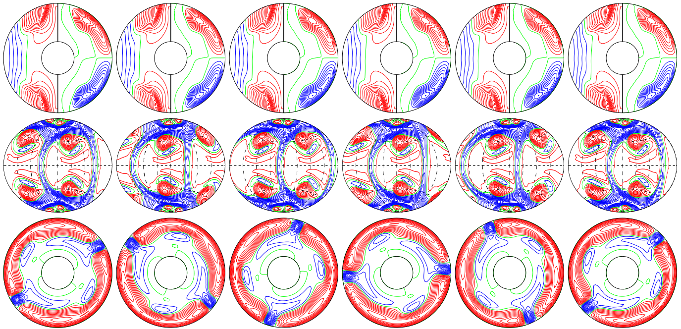
a.e03p1t03r-100000m1n2N3z2.15e5 E_{\text{kin}}
