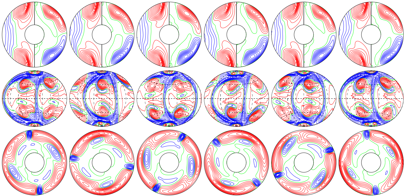
a.e03p1t03r-100000m1n2N3z2.55e5 E_{\text{kin}}
