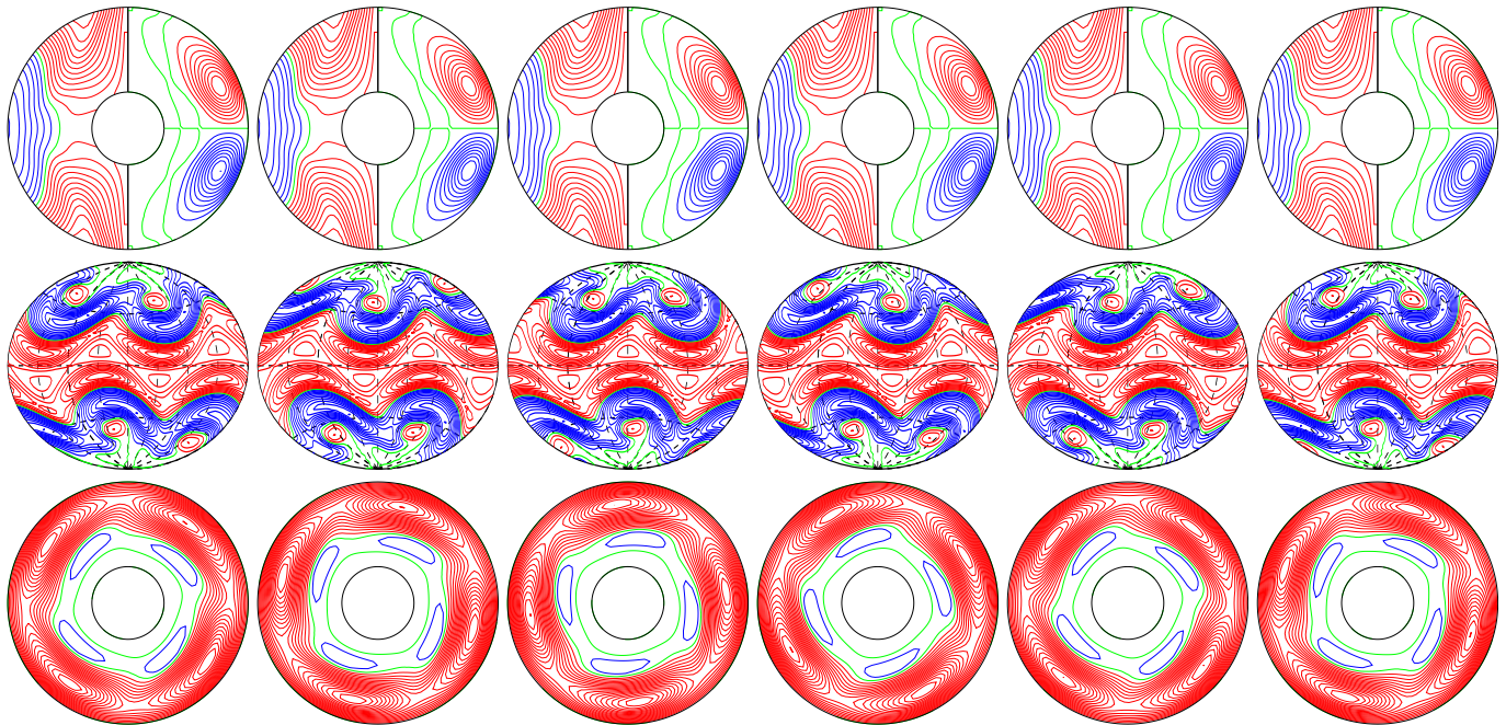
a.e03p1t03r-100000m1n2N1z2.1e5 E_{\text{kin}}
