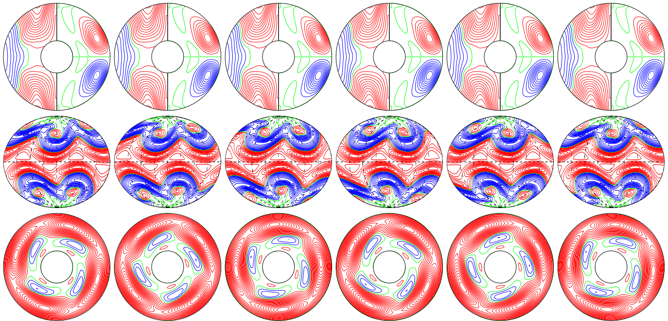
a.e03p1t03r-100000m1n2N1z2.5e5 E_{\text{kin}}
