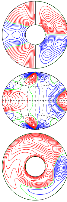
a.e03p1t03r-30000m1n2N0001z2.5e5 E_{\text{kin}}
