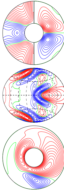
a.e03p1t03r-10000m1n2N0001z2e5 E_{\text{kin}}
