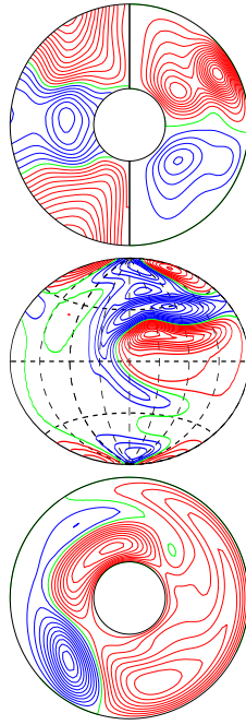
a.e03p1t03r-30000m1n2N0001z2.36e5 E_{\text{kin}}
