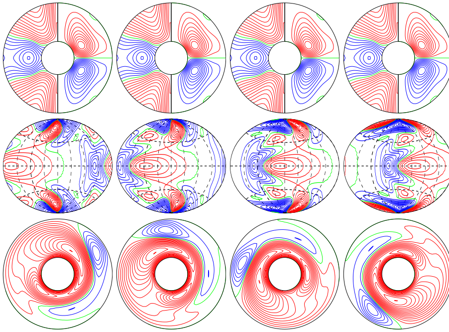
a.e03p1t03r-10000m1n2N0001z1.8e5 E_{\text{kin}}
