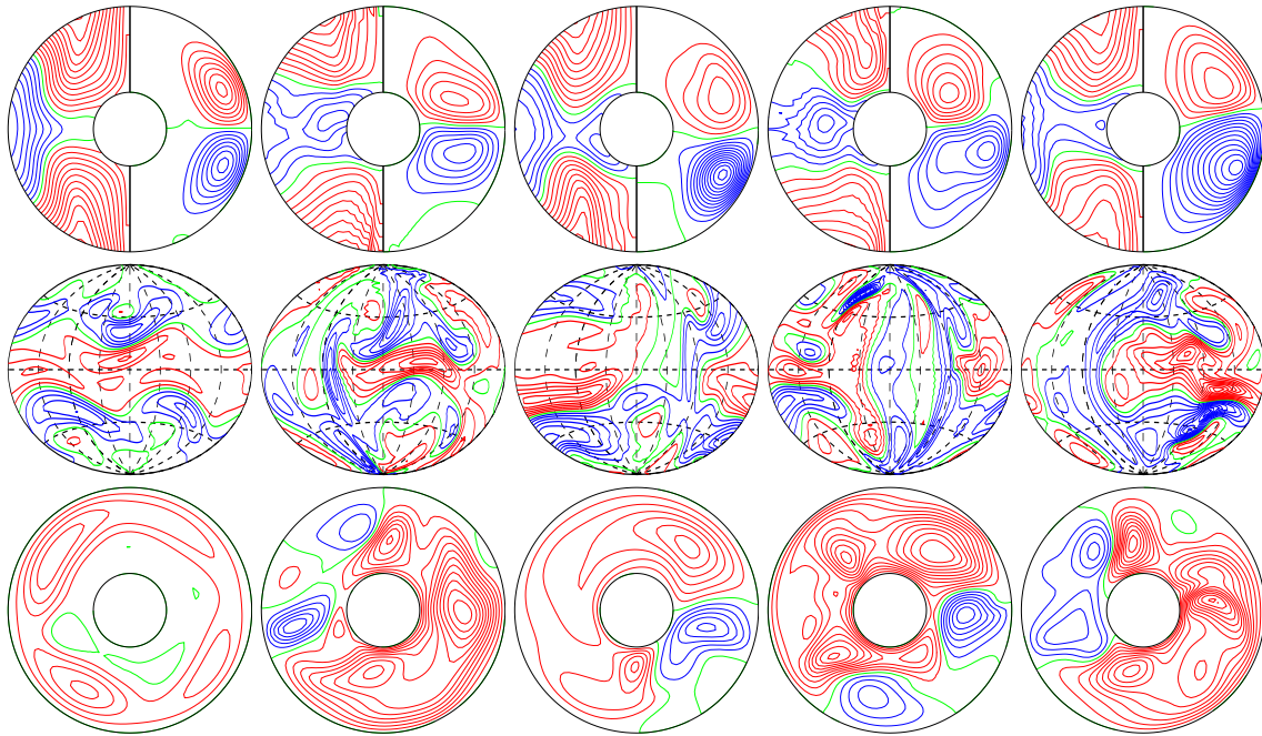
a.e03p1t03r-10000m1n2N0001z2.5e5 E_{\text{kin}}
