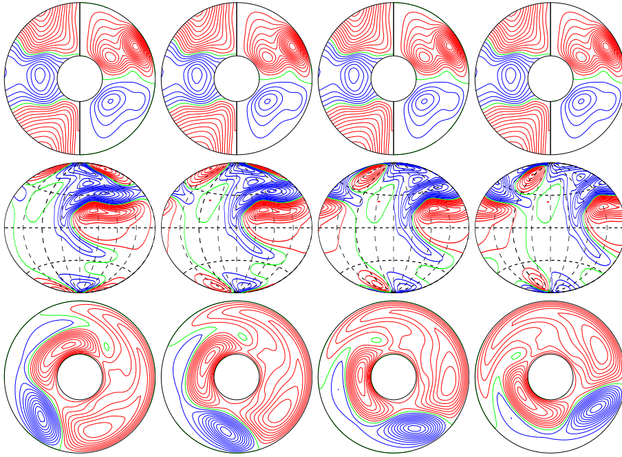
a.e03p1t03r-30000m1n2N0001z2.36e5 E_{\text{kin}}
