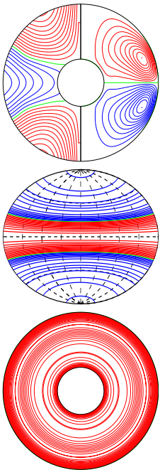
a.e03p1t03r-100000m1n2N0001z3.3e5 E_{\text{kin}}
