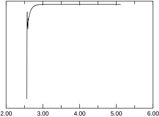
E_{kin,asymm.}
