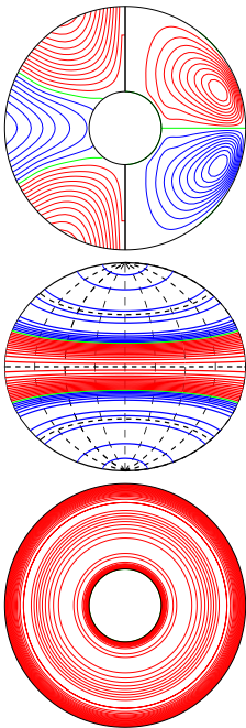
a.e03p1t03r-100000m1n2N0001z3.1e5 E_{\text{kin}}
