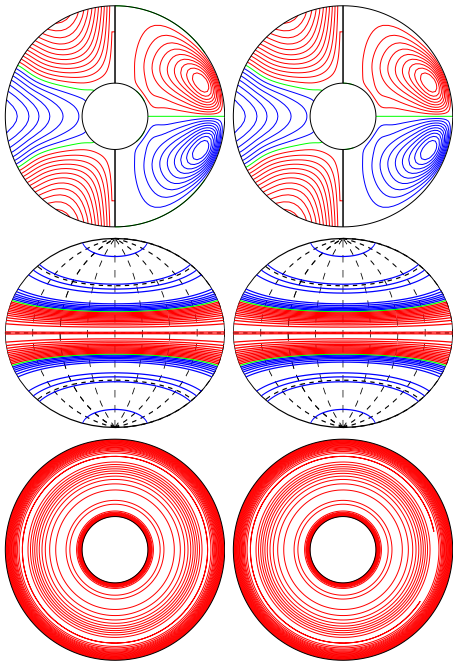
a.e03p1t03r-100000m1n2N0001z3.2e5 E_{kin}
