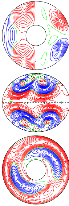
a.e03p1t03r-100000m1n2N1z2.4e5a E_{\text{kin}}
