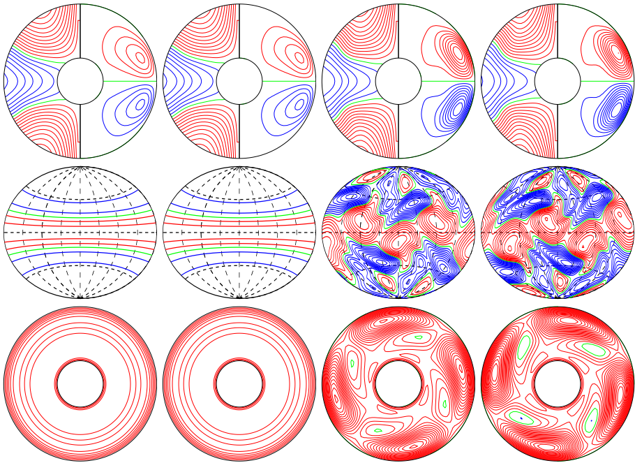
a.e03p1t03r-100000m1n2N0001z3.2e5 E_{\text{kin}}
