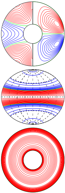
a.e03p1t03r-100000m1n2N0001z2.95e5 E_{\text{kin}}
