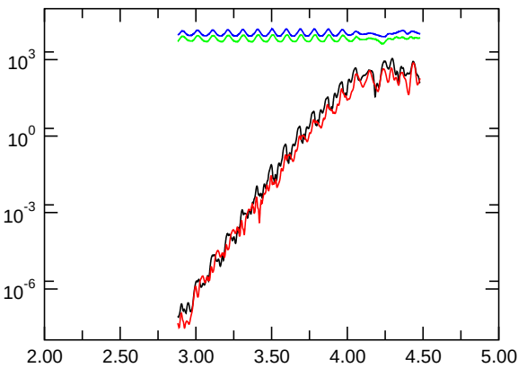
E_{kin,asymm.}
