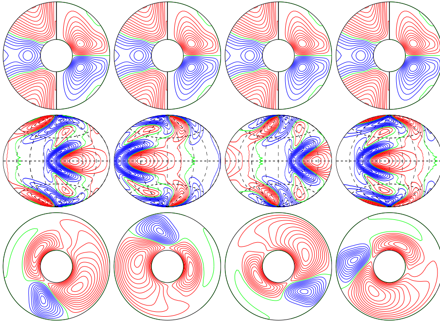
a.e03p1t03r-10000m1n2N0001z2.08e5 E_{\text{kin}}
