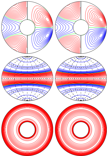
a.e03p1t03r-100000m1n2N0001z3.1e5 E_{\text{kin}}
