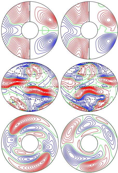
a.e03p1t03r-100000m1n2N0001z3.55e5 E_{kin}
