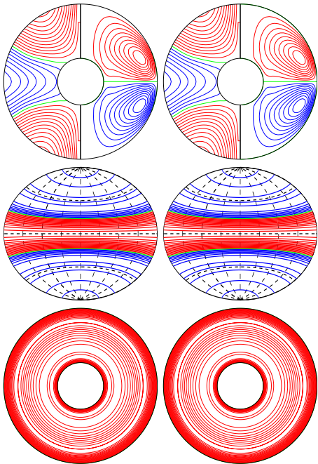
a.e03p1t03r-100000m1n2N0001z3.05e5 E_{\text{kin}}
