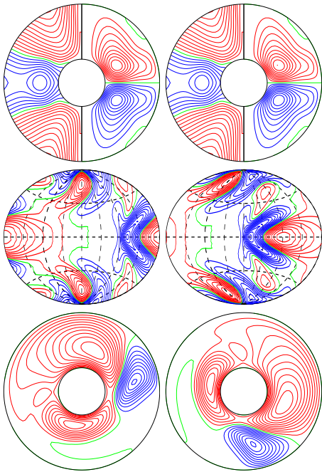
a.e03p1t03r-10000m1n2N0001z2.06e5 E_{\text{kin}}
