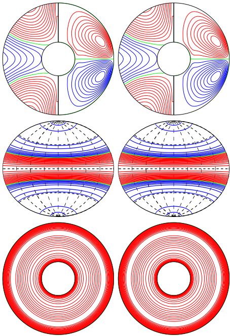
a.e03p1t03r-100000m1n2N0001z2.95e5 E_{\text{kin}}
