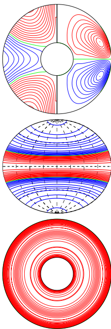
a.e03p1t03r-100000m1n2N0001z3.3e5 E_{\text{kin}}
