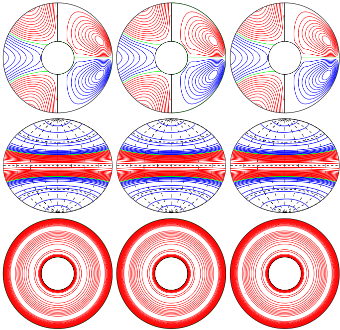
a.e03p1t03r-100000m1n2N0001z3.05e5 E_{\text{kin}}
