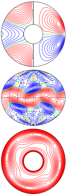
a.e03p1t03r-100000m1n2N0001z2.94e5a E_{\text{kin}}
