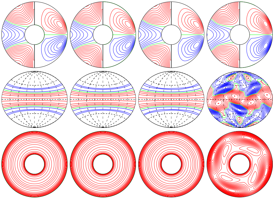
a.e03p1t03r-100000m1n2N0001z3.05e5 E_{\text{kin}}
