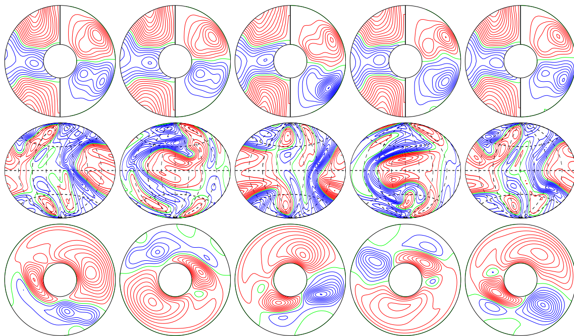
a.e03p1t03r-10000m1n2N0001z2.11e5 E_{\text{kin}}
