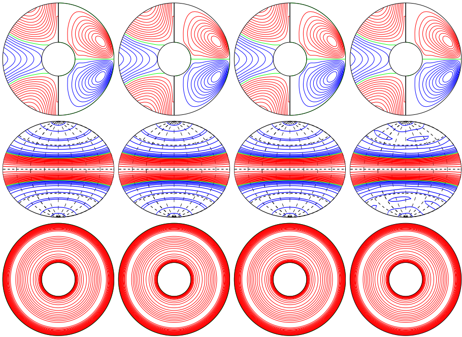
a.e03p1t03r-100000m1n2N0001z2.95e5 E_{\text{kin}}
