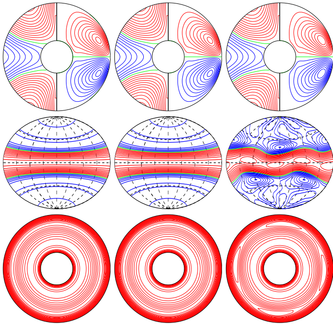
a.e03p1t03r-100000m1n2N0001z3.1e5 E_{\text{kin}}
