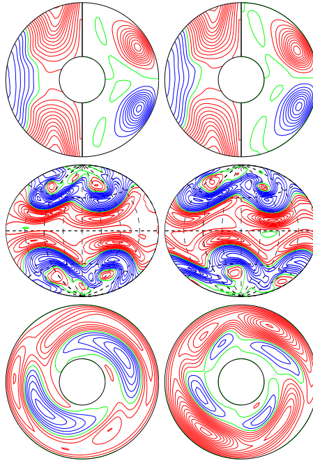
a.e03p1t03r-100000m1n2N1z2.4e5a E_{\text{kin}}
