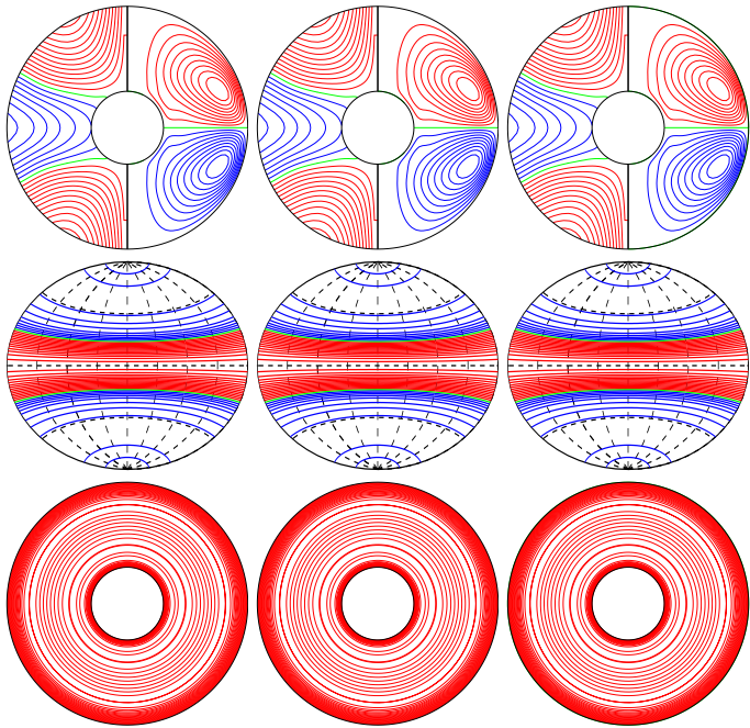
a.e03p1t03r-100000m1n2N0001z2.9e5 E_{\text{kin}}
