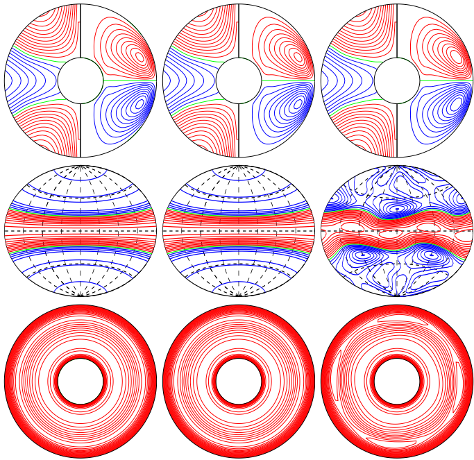
a.e03p1t03r-100000m1n2N0001z3.1e5 E_{\text{kin}}
