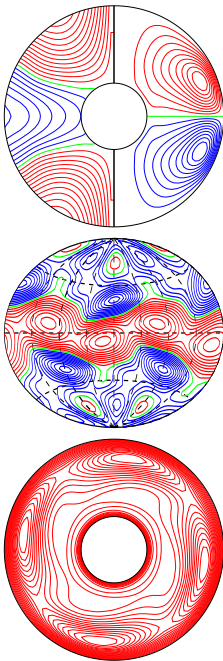
a.e03p1t03r-100000m1n2N0001z2.94e5a E_{\text{kin}}
