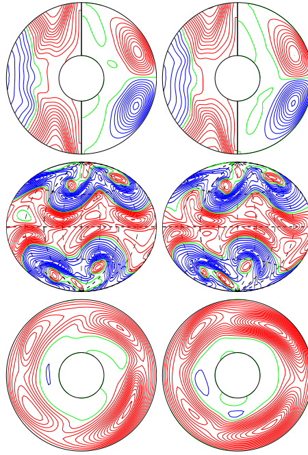
a.e03p1t03r-50000m1n2Nz2.0e5a E_{\text{kin}}
