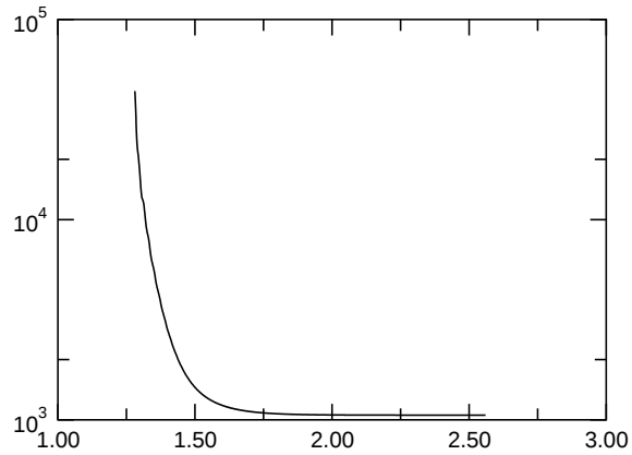
E_{kin,asymm.}
