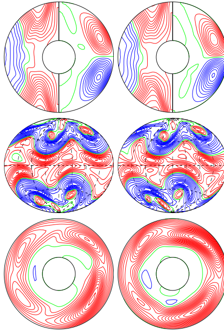
a.e03p1t03r-50000m1n2Nz2.0e5a E_{\text{kin}}
