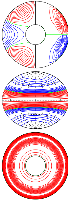
a.e03p1t03r-50000m1n2N2z1.0e5a E_{\text{kin}}
