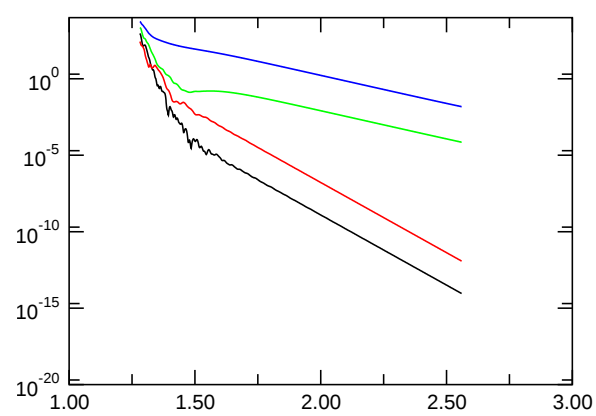
E_{kin,asymm.}
