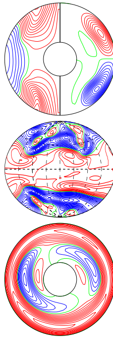
a.e03p1t03r-50000m1n2N2z1.2e5a E_{\text{kin}}
