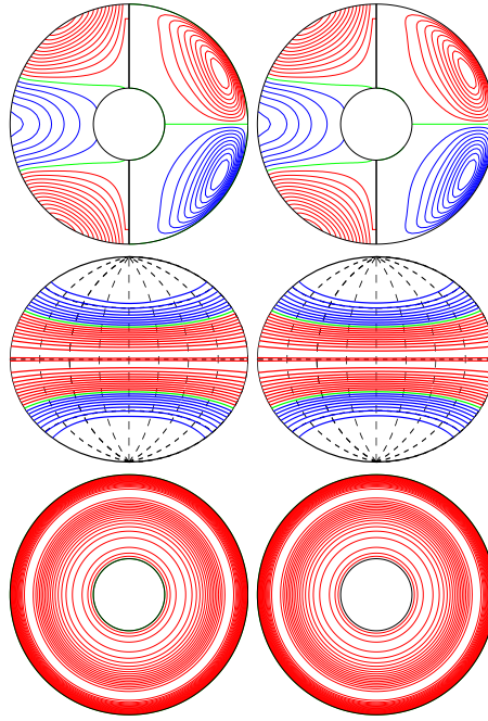
a.e03p1t03r-50000m1n2N2z0.4e5a E_{\text{kin}}
