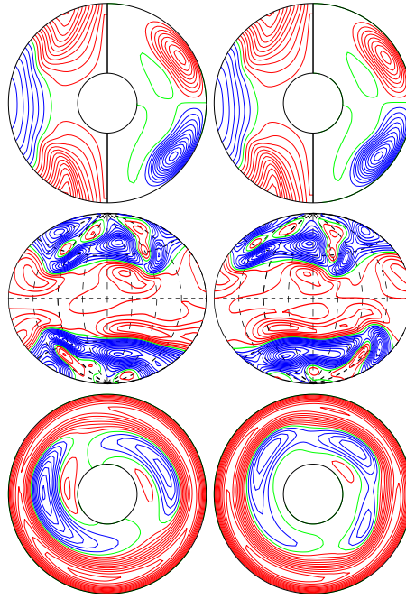
a.e03p1t03r-50000m1n2N2z1.2e5a E_{\text{kin}}
