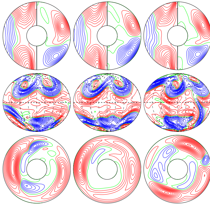
a.e03p1t03r-50000m1n2N2z1.8e5a E_{\text{kin}}
