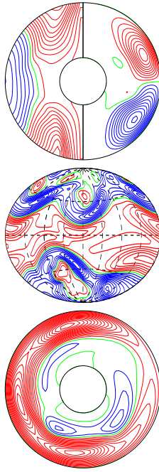
a.e03p1t03r-50000m1n2N2z1.4e5a E_{\text{kin}}
