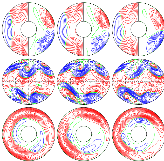
a.e03p1t03r-50000m1n2N2z1.5e5a E_{\text{kin}}
