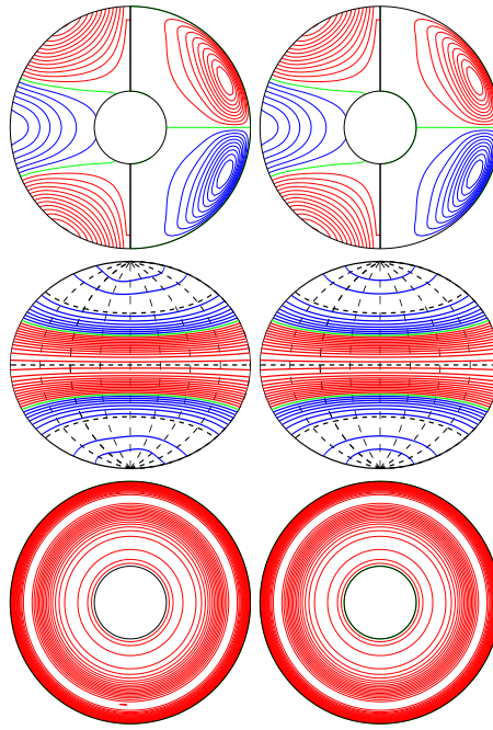
a.e03p1t03r-50000m1n2N2z0.6e5a E_{\text{kin}}
