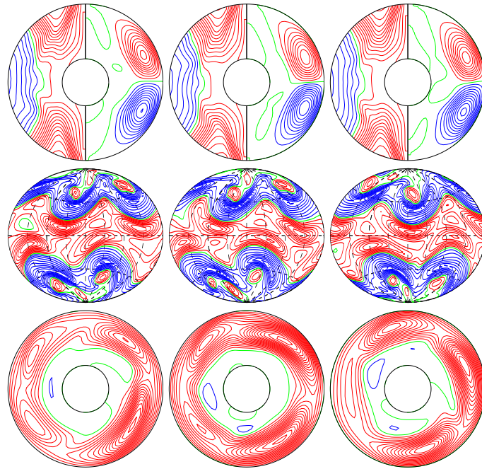
a.e03p1t03r-50000m1n2Nz2.0e5a E_{\text{kin}}
