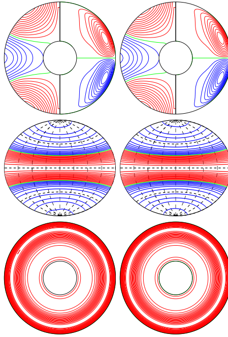
a.e03p1t03r-50000m1n2N2z0.8e5a E_{\text{kin}}
