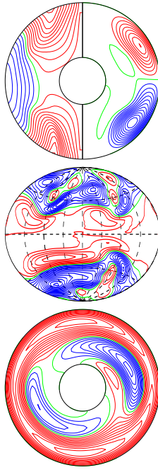
a.e03p1t03r-50000m1n2N2z1.25e5a E_{\text{kin}}
