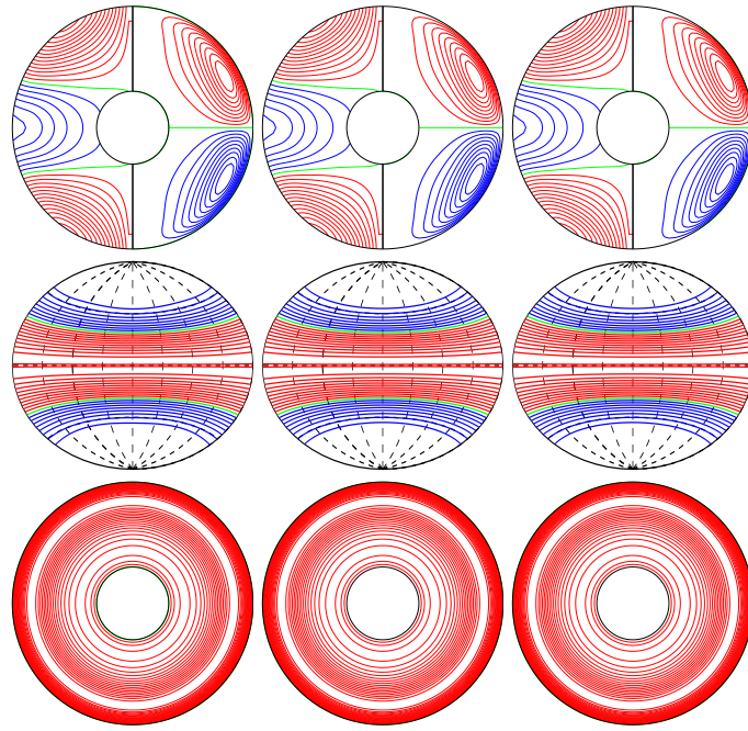
a.e03p1t03r-50000m1n2N2z0.4e5a E_{\text{kin}}
