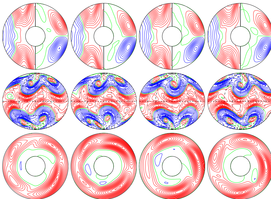
a.e03p1t03r-50000m1n2Nz2.0e5a E_{\text{kin}}
