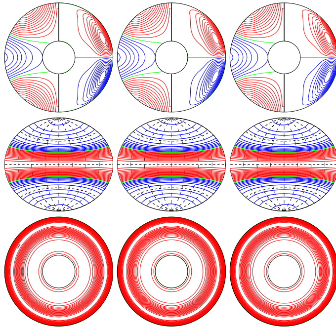
a.e03p1t03r-50000m1n2N2z0.8e5a E_{\text{kin}}
