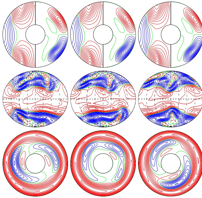
a.e03p1t03r-50000m1n2N2z1.2e5a E_{\text{kin}}
