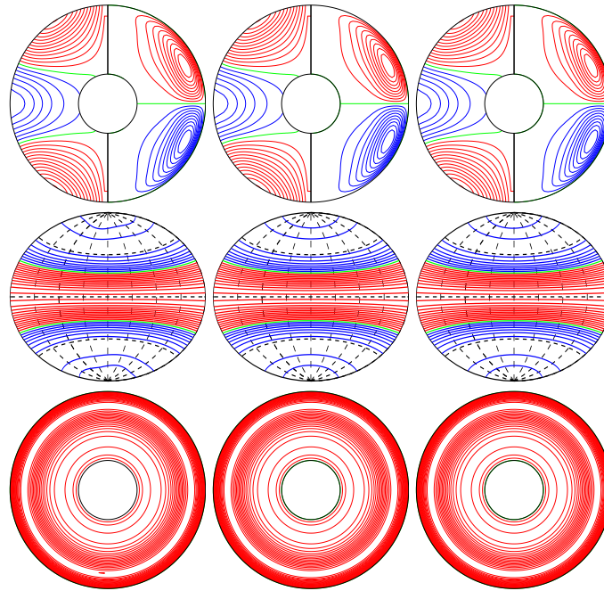
a.e03p1t03r-50000m1n2N2z0.6e5a E_{\text{kin}}
