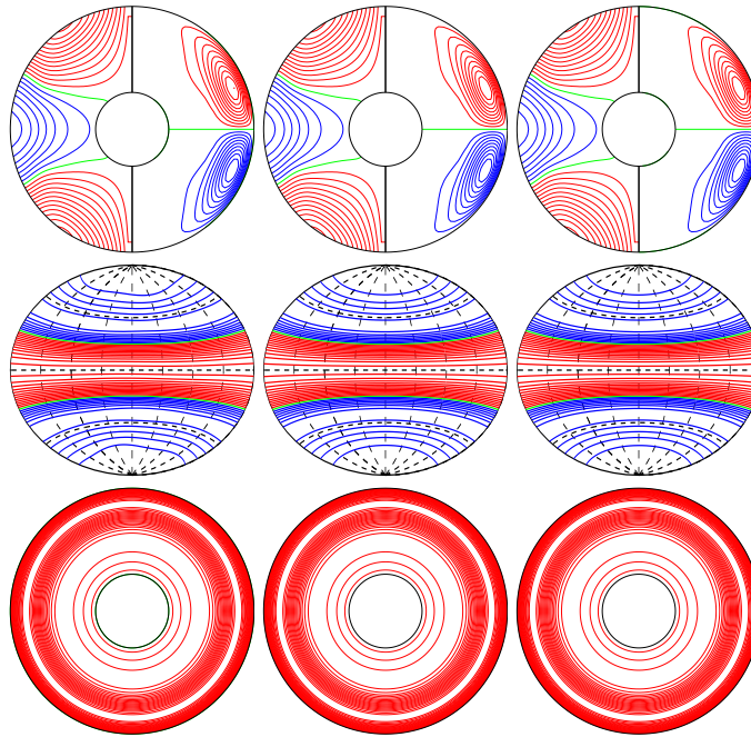
a.e03p1t03r-50000m1n2N2z1.0e5a E_{\text{kin}}
