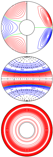
a.e03p1t03r-50000m1n2N2z1.05e5a E_{\text{kin}}
