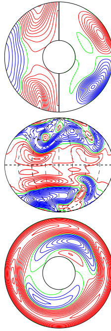
a.e03p1t03r-50000m1n2N2z1.3e5a E_{\text{kin}}
