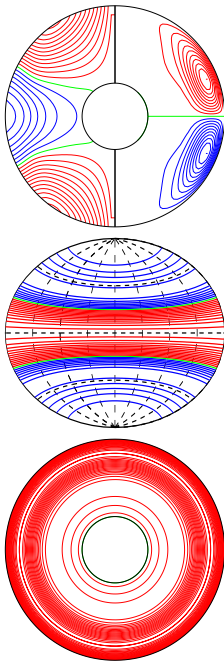
a.e03p1t03r-50000m1n2N2z1.0e5ac E_{\text{kin}}
