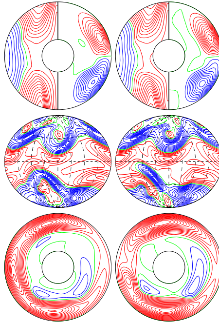
a.e03p1t03r-50000m1n2N2z1.4e5a E_{\text{kin}}
